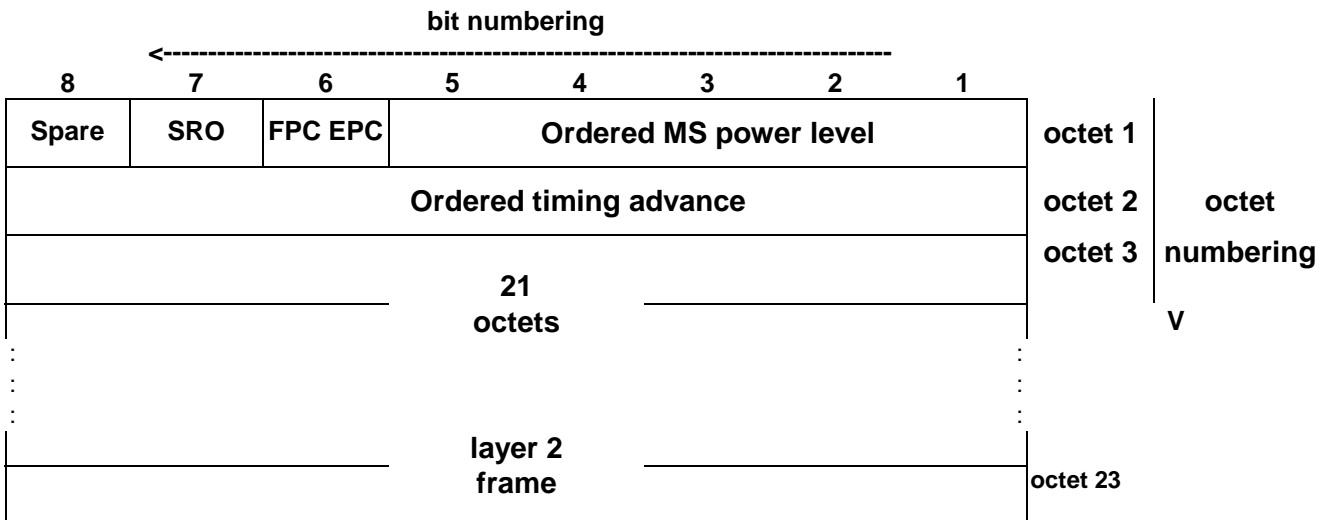
Figure 7.1.1: SACCH downlink block format for MS operating in A/Gb mode
