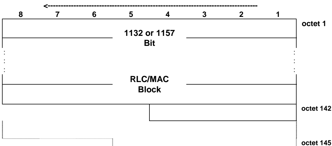
Figure 7.6.12.2: PDTCH block type 12 (MCS-8) downlink format
