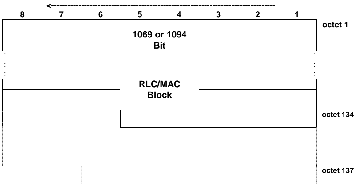
Figure 7.6.15.1: PDTCH block type 15 (UAS-8) format
