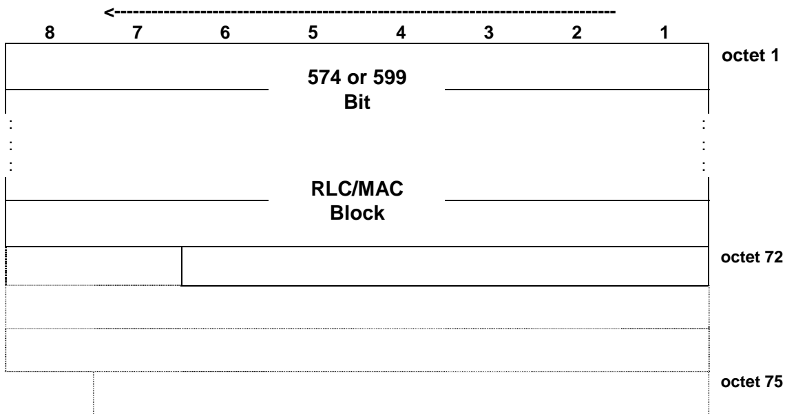
Figure 7.6.28.1: PDTCH block type 28 (DAS-6) format
