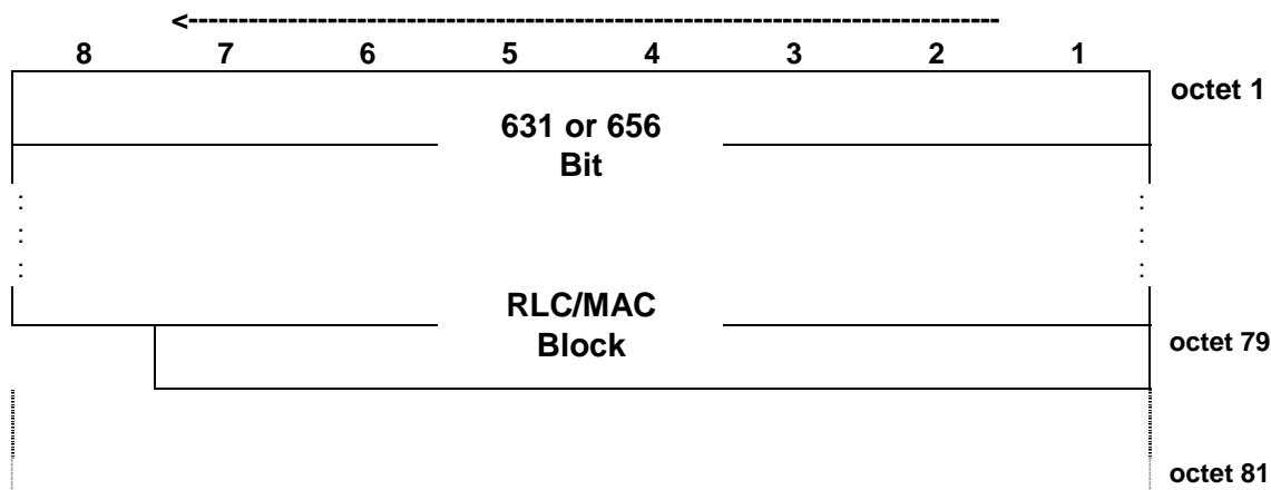
Figure 7.6.10.1: PDTCH block type 10 (MCS-6) uplink format
