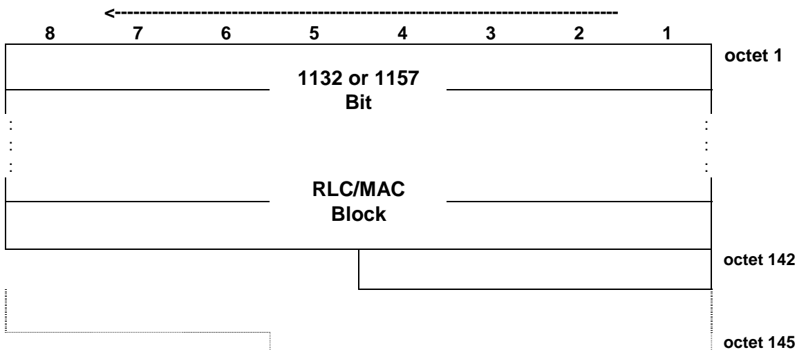
Figure 7.6.12.2: PDTCH block type 12 (MCS-8) downlink format
