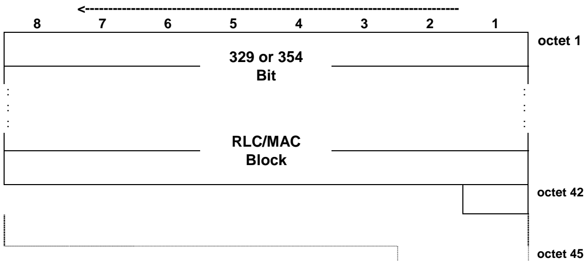
Figure 7.6.7: PDTCH block type 7 (MCS-3) format
