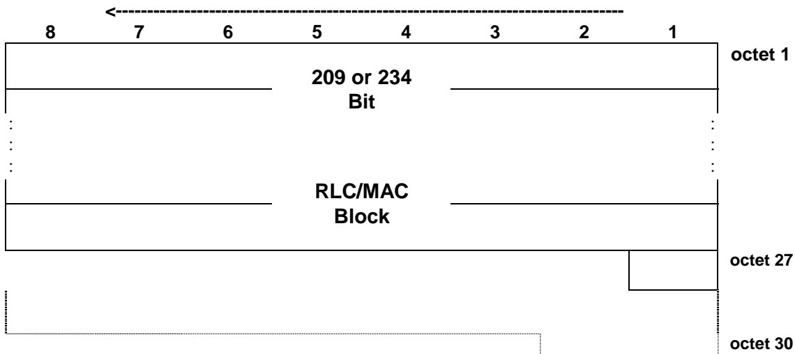
Figure 7.6.5: PDTCH block type 5 (MCS-1) format
