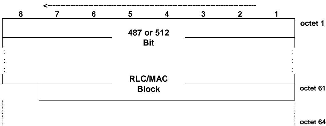
Figure 7.6.9.1: PDTCH block type 9 (MCS-5) uplink format
