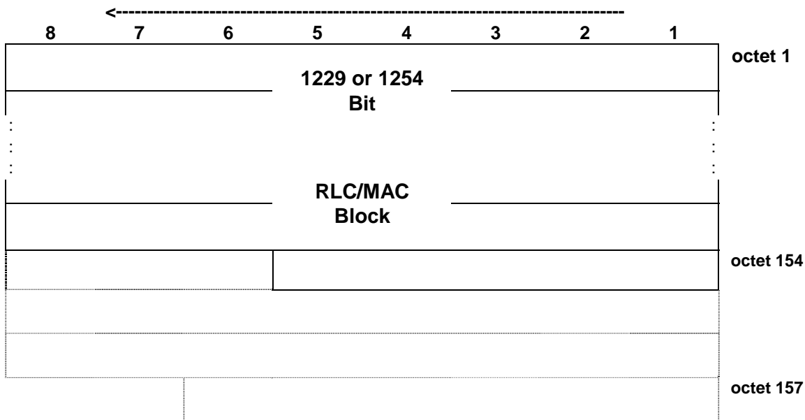
Figure 7.6.16.1: PDTCH block type 16 (UAS-9) format
