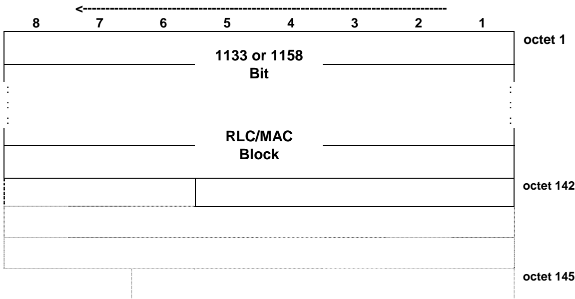
Figure 7.6.31.1: PDTCH block type 31 (DAS-9) format
