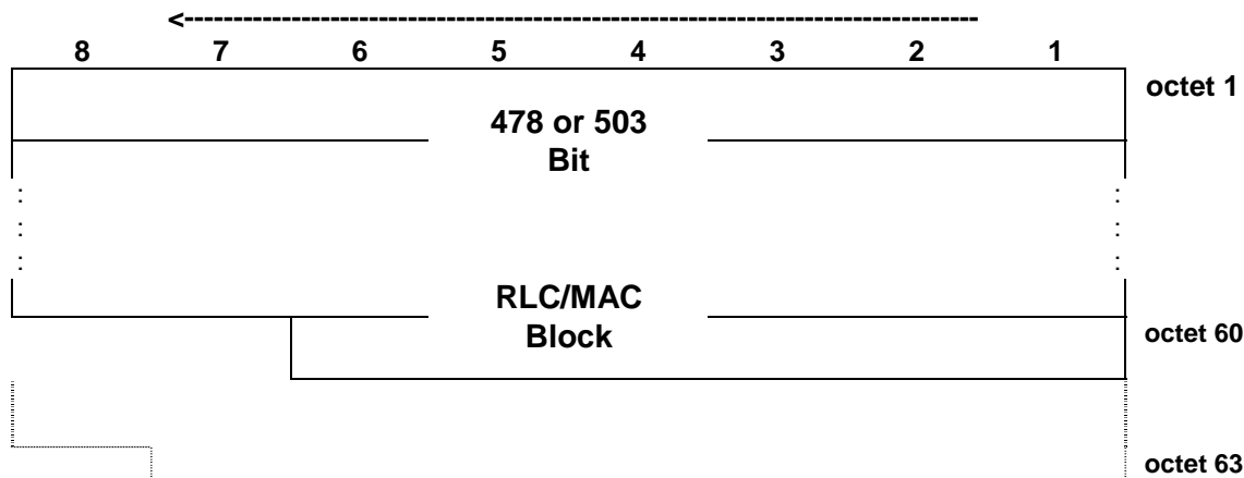
Figure 7.6.9.2: PDTCH block type 9 (MCS-5) downlink format
