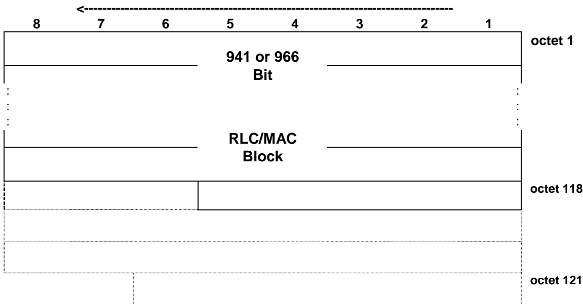
Figure 7.6.30.1: PDTCH block type 30 (DAS-8) format
