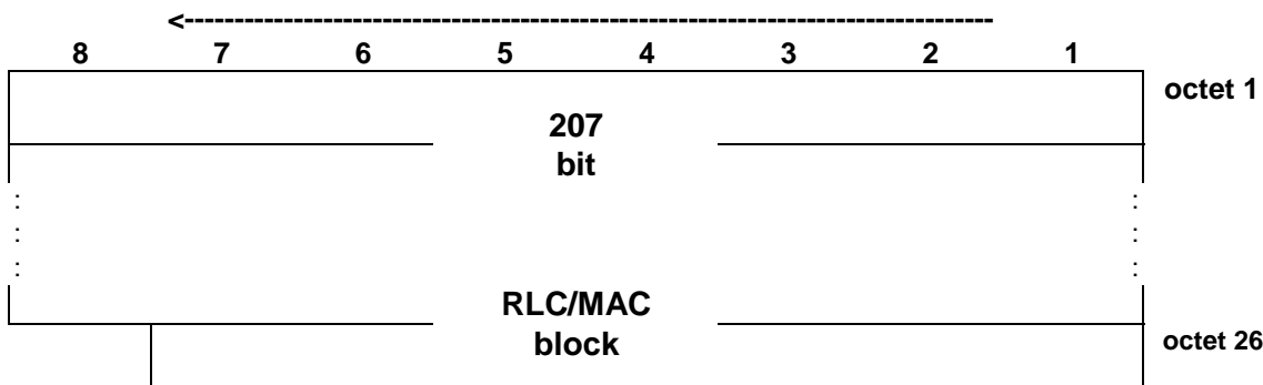
Figure 7.5a: PACCH downlink block format for MCS-0
