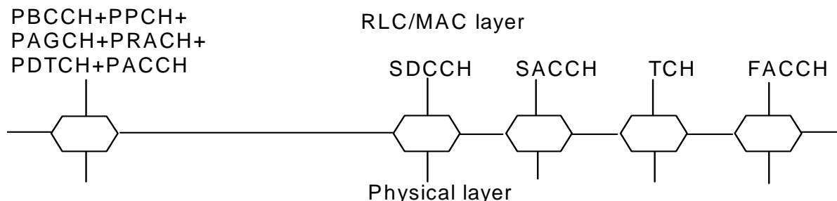
Figure 3.1.d: SAP between the physical layer and the RLC/MAC layer when the MS is operating in Iu mode
