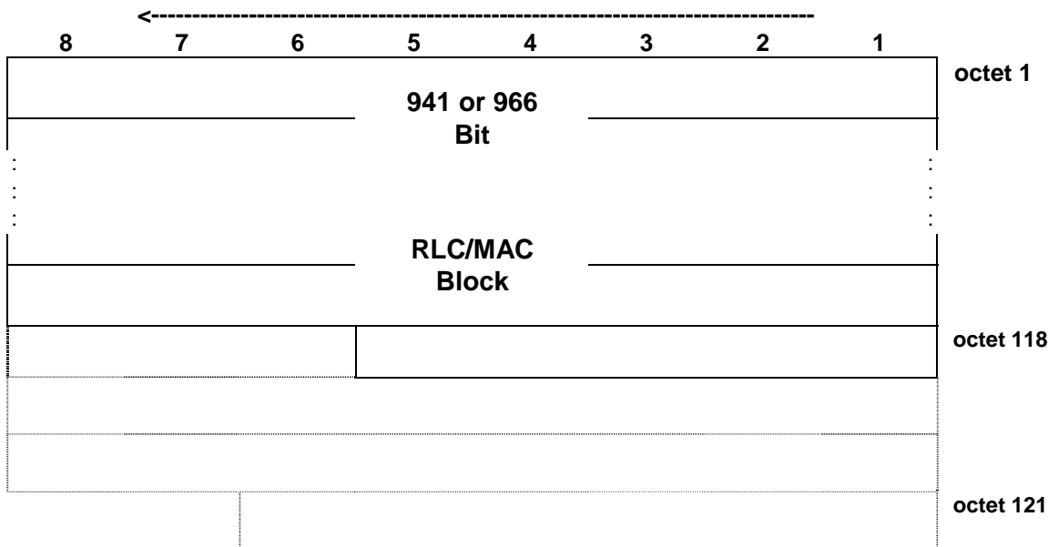
Figure 7.6.14.1: PDTCH block type 14 (UAS-7) format
