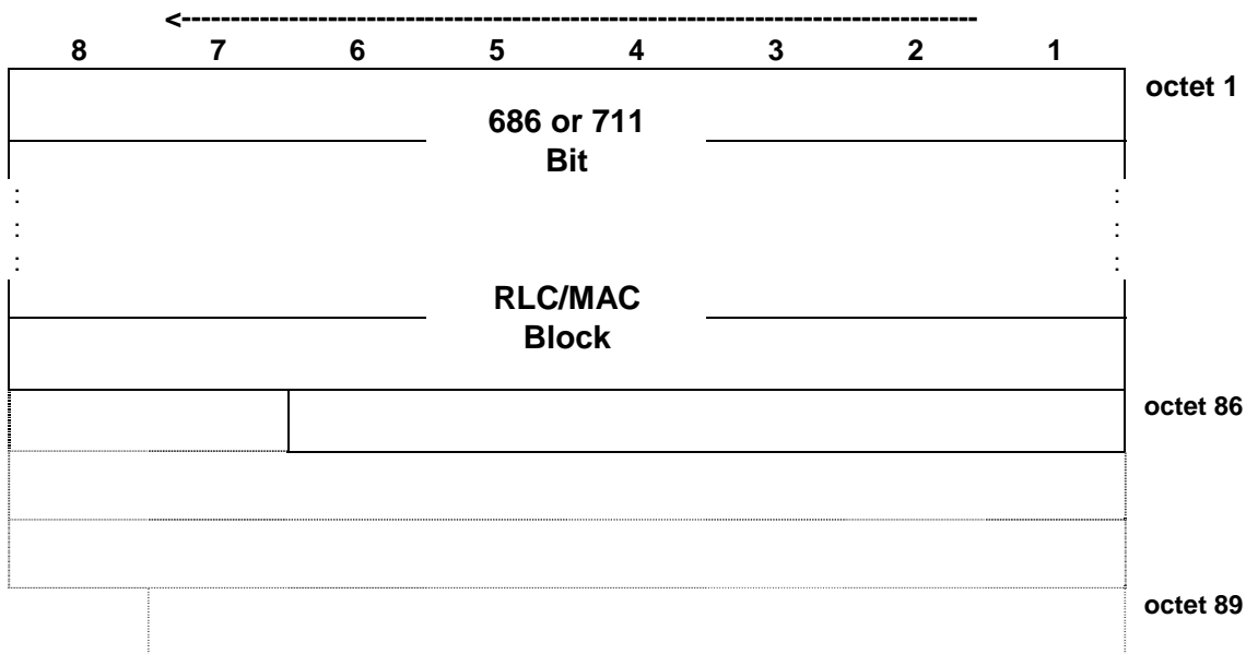
Figure 7.6.29.1: PDTCH block type 29 (DAS-7) format
