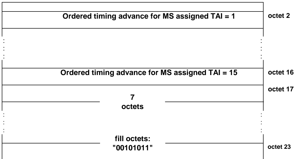
Figure 7.8: PTCCH downlink block format
