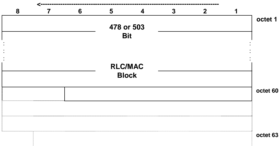
Figure 7.6.27.1: PDTCH block type 27 (DAS-5) format
