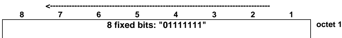
Figure 7.9.a: PTCCH uplink block format
