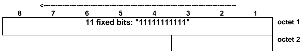
Figure 7.9.b (sheet 2 of 2): PTCCH uplink block format
