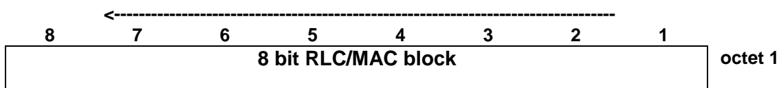
Figure 7.7.a (sheet 1 of 2): PRACH uplink/PACCH uplink short acknowledgement block format
