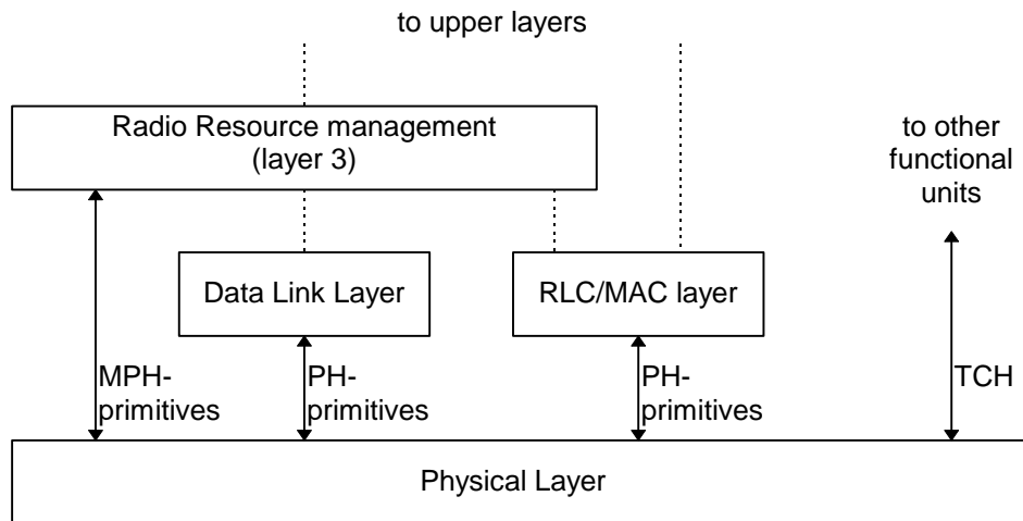
Figure 2: Interfaces with the Physical Layer
