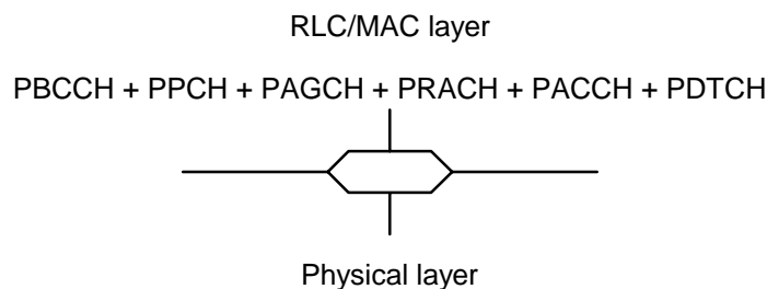
Figure 3.1.c: SAP between the physical layer and the RLC/MAC layer in the MS
