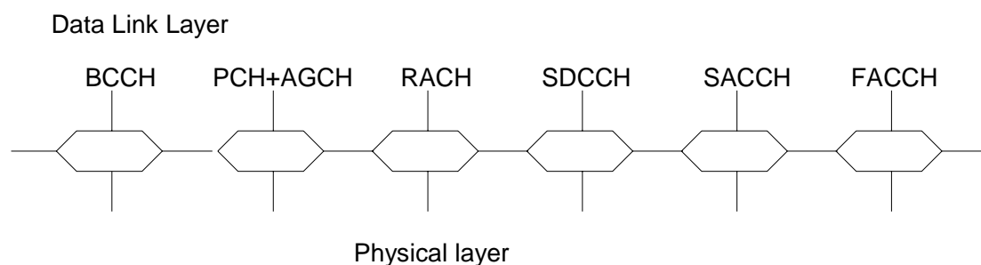
Figure 3.1.b: SAPs between the physical layer and the data link layer in the MS
