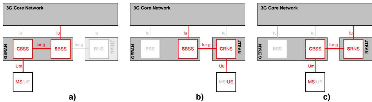
Figure 2: Scenarios using the Iur-g interface.
