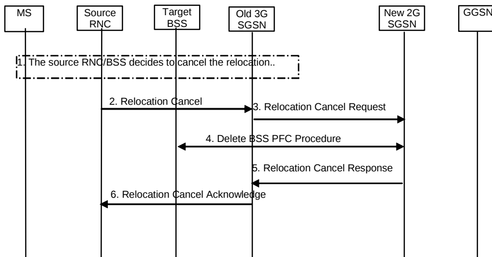
Figure 20b: Relocation Cancel; Inter-SGSN case, UTRAN/GERAN lu mode→ GERAN A/Gb mode
