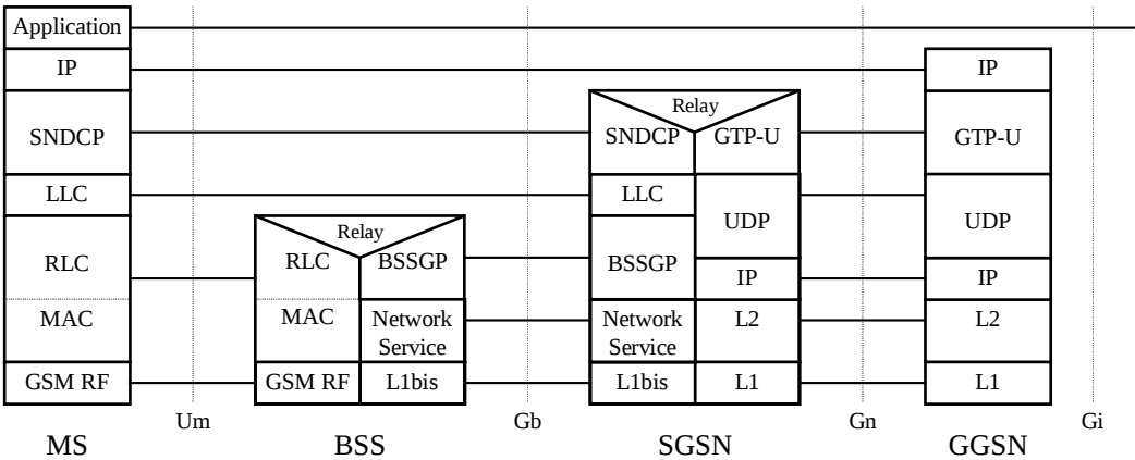
Figure 2: User Plane protocol architecture in A/Gb mode
