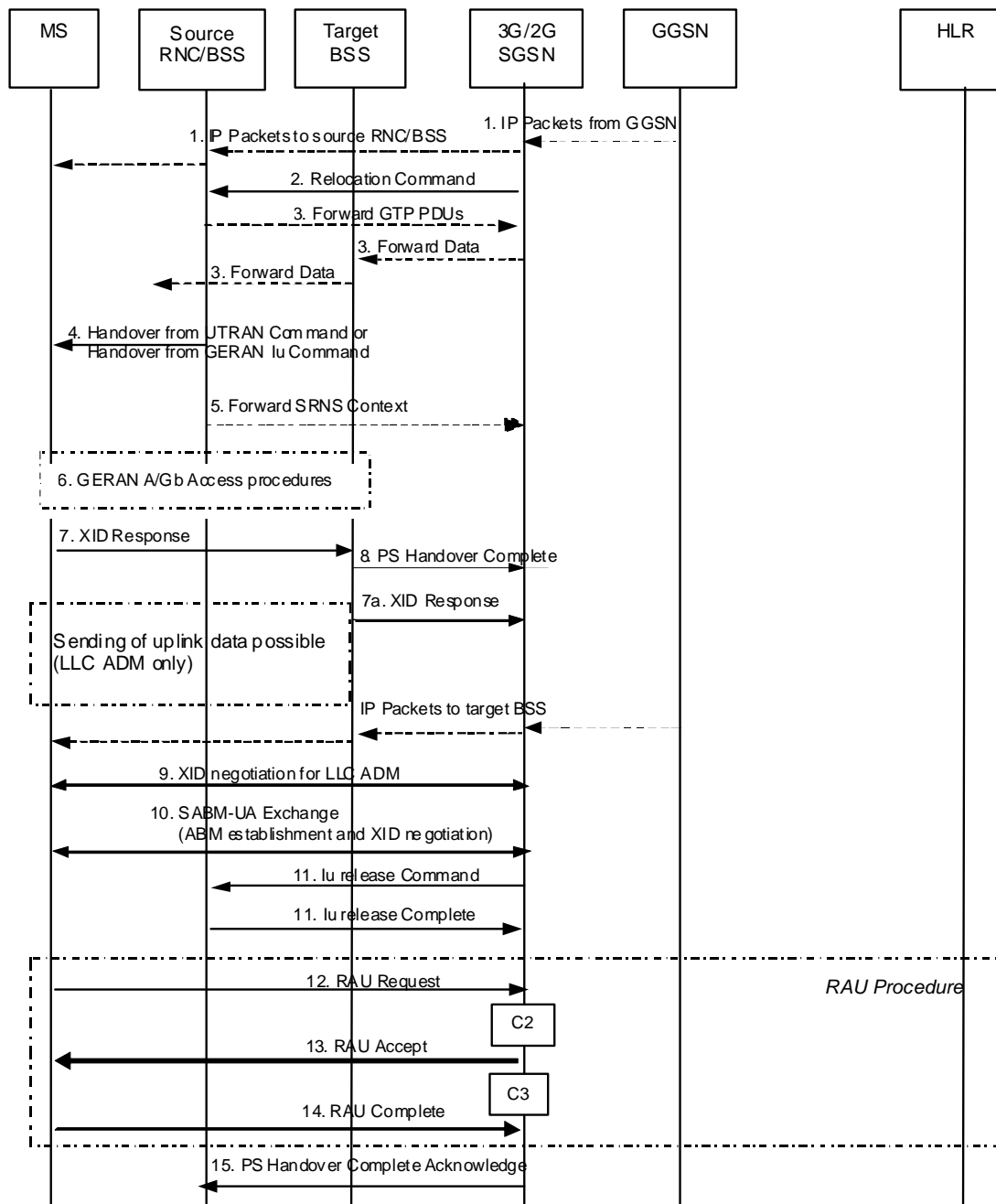
Figure 16: PS Handover Execution Phase; Inter-RAT/mode, Intra-SGSN case (UTRAN/GERAN Iu mode → GERAN A/Gb mode)
