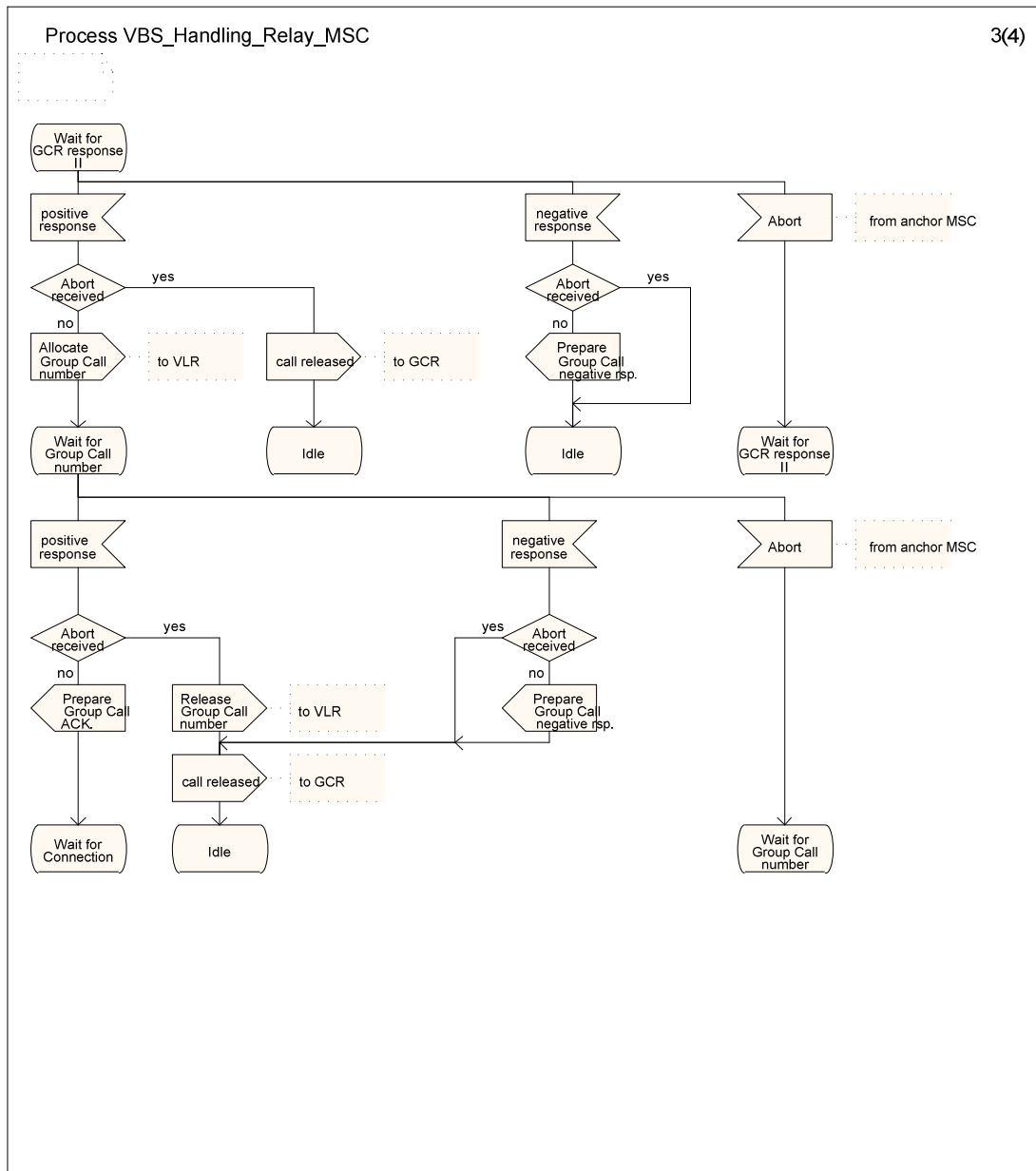
Figure 7: VBS handling process in the relay MSC (sheet 3 of 4)
