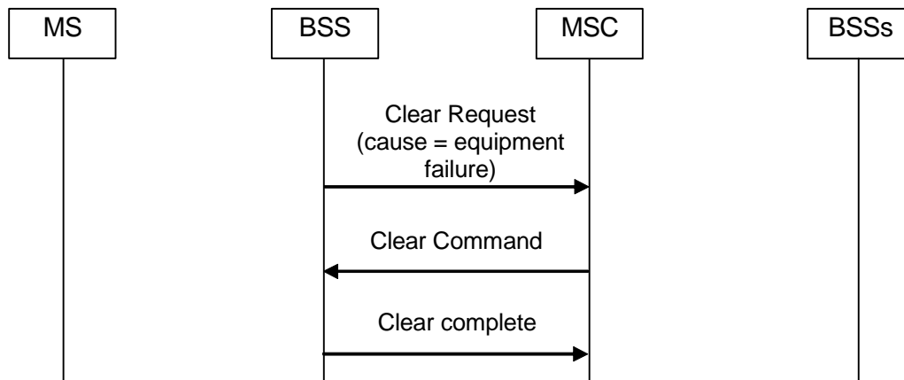
Figure 4f: A-interface link sharing used or broadcast call re-establishment by the BSS supported: release after equipment failure concerning the link between MSC and BSS
