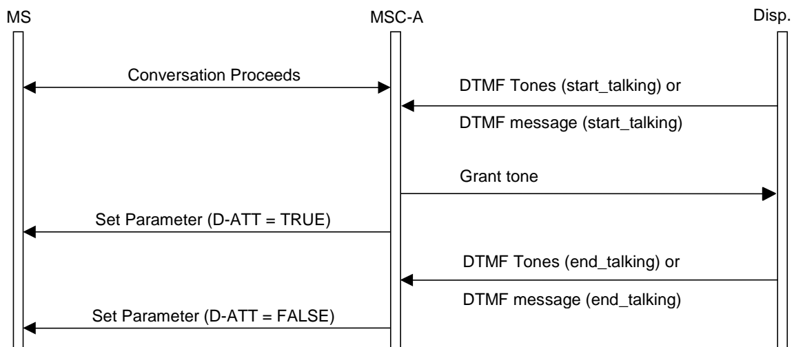
Figure 5b: Signalling information required when the talker is attached to the Anchor MSC and a dispatcher sends DTMF signals
