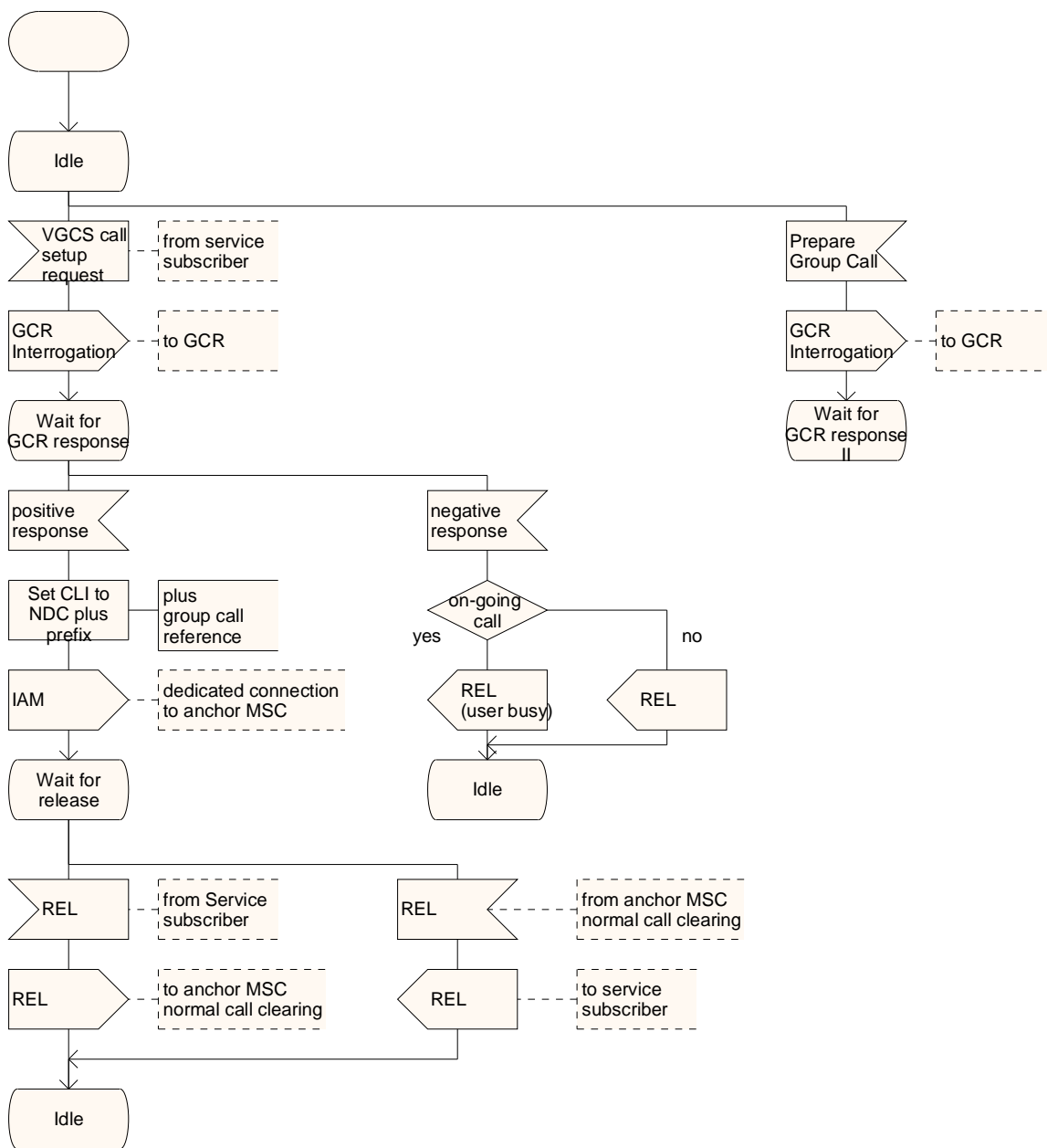
Figure 10: The VGCS handling process in the relay MSC (sheet 1 of 7)
