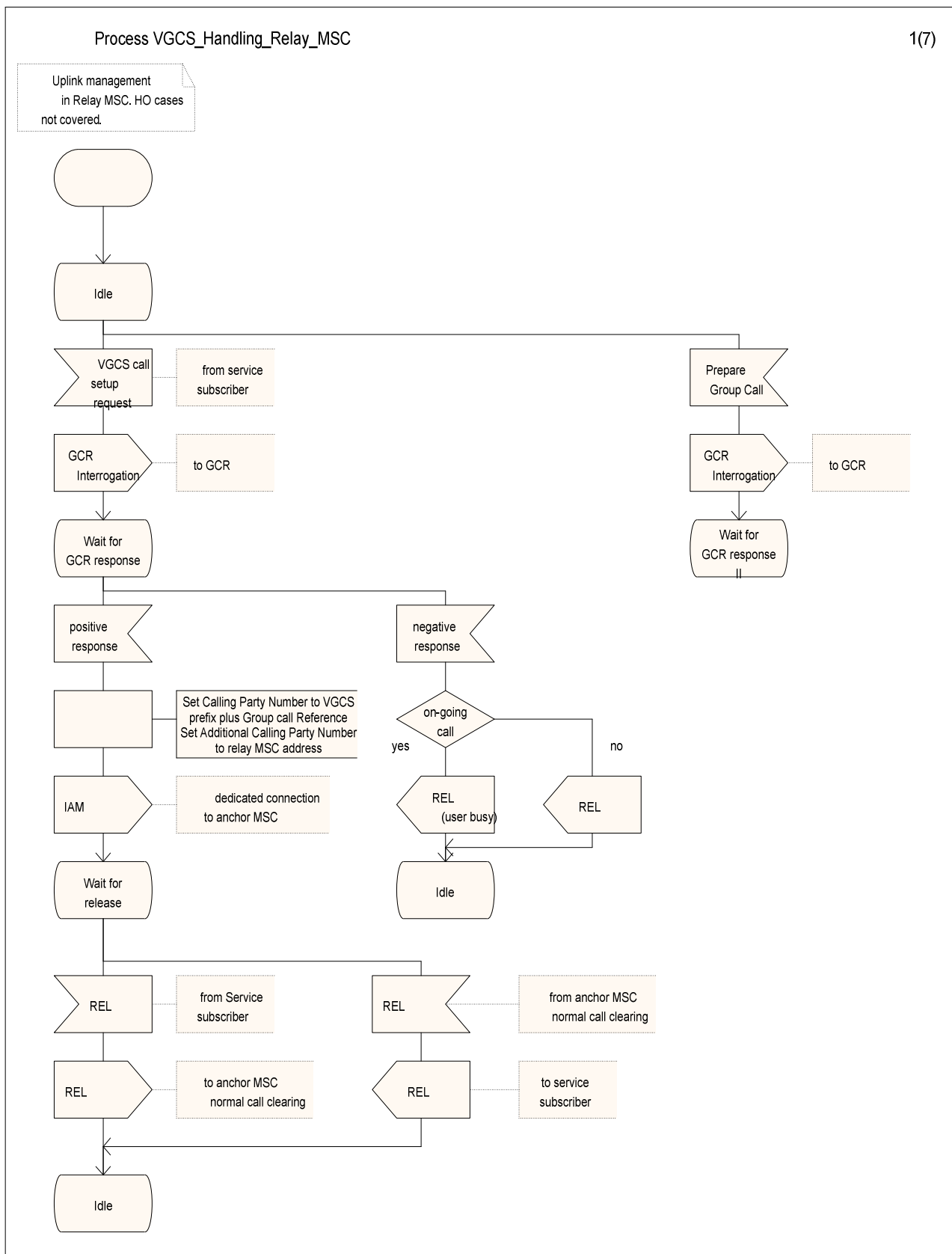
Figure 10: The VGCS handling process in the relay MSC (sheet 1 of 7)
