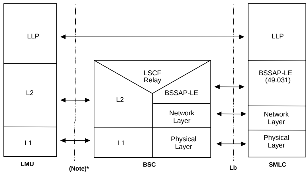
Figure 9: Signalling between an SMLC and Type B LMU
