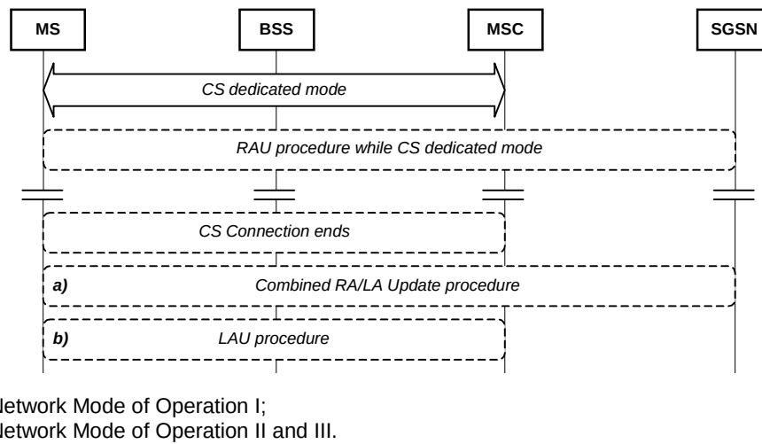
Figure 16: LA Update and RA Update procedures in CS dedicated mode, packet idle mode and Ready state
