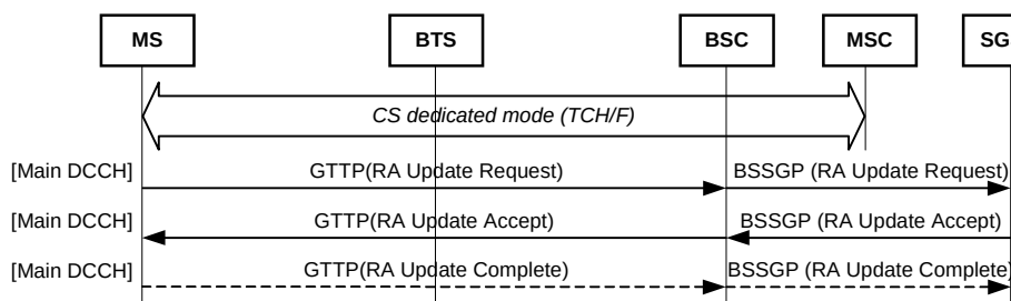
Figure 14: Routeing Area Update procedure in dedicated mode, packet idle mode and Ready state; performed on the main DCCH
