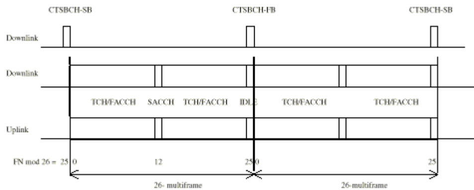
Figure 2: 26-multiframe structure
