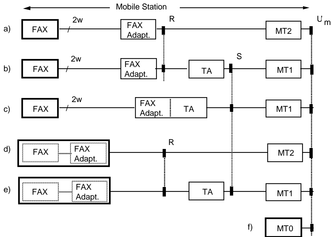
Figure 2/43.045: Reference configurations
