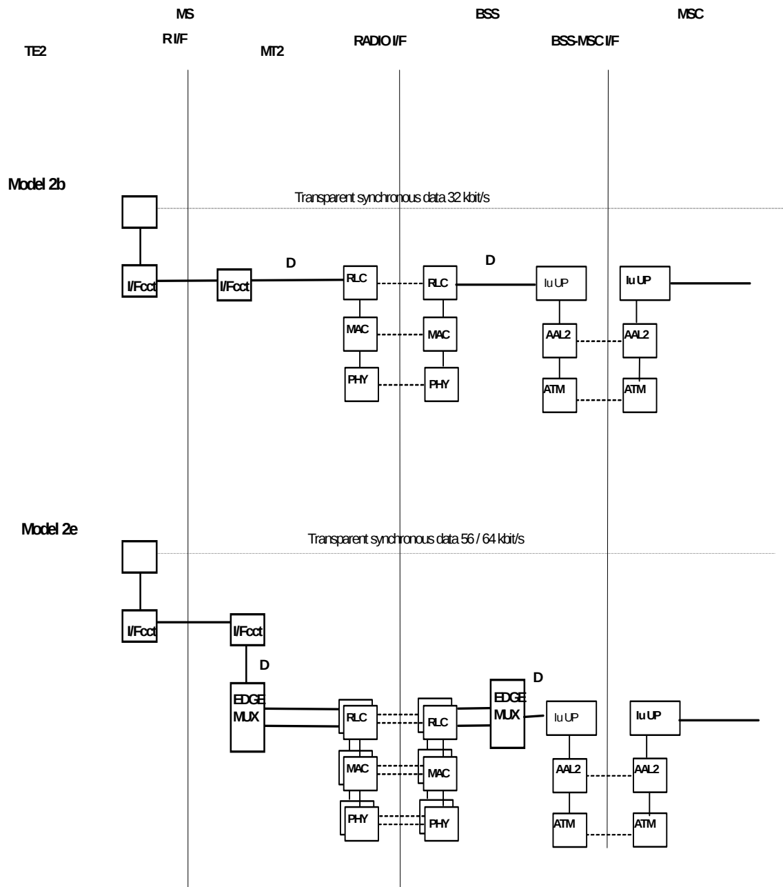
Figure 13: Information transfer protocol models for PLMN connections using TCH/F32.0 EDGE channels
