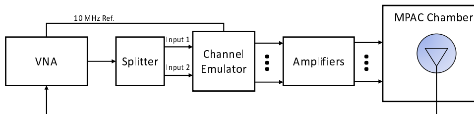
Figure C.3.2-2: Setup for Beam-Specific PDP measurements (Beam 1)
