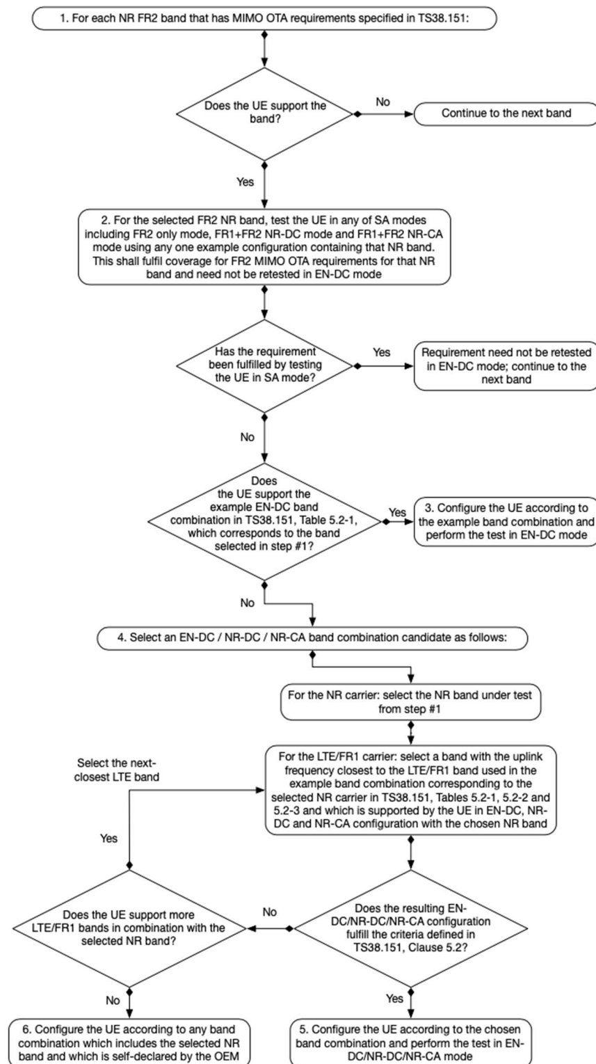
Figure 5.2-2: Decision tree for FR2 MIMO OTA testing
