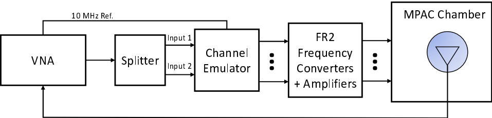
Figure I.3.2-1: Setup for PDP measurements (FR2)
