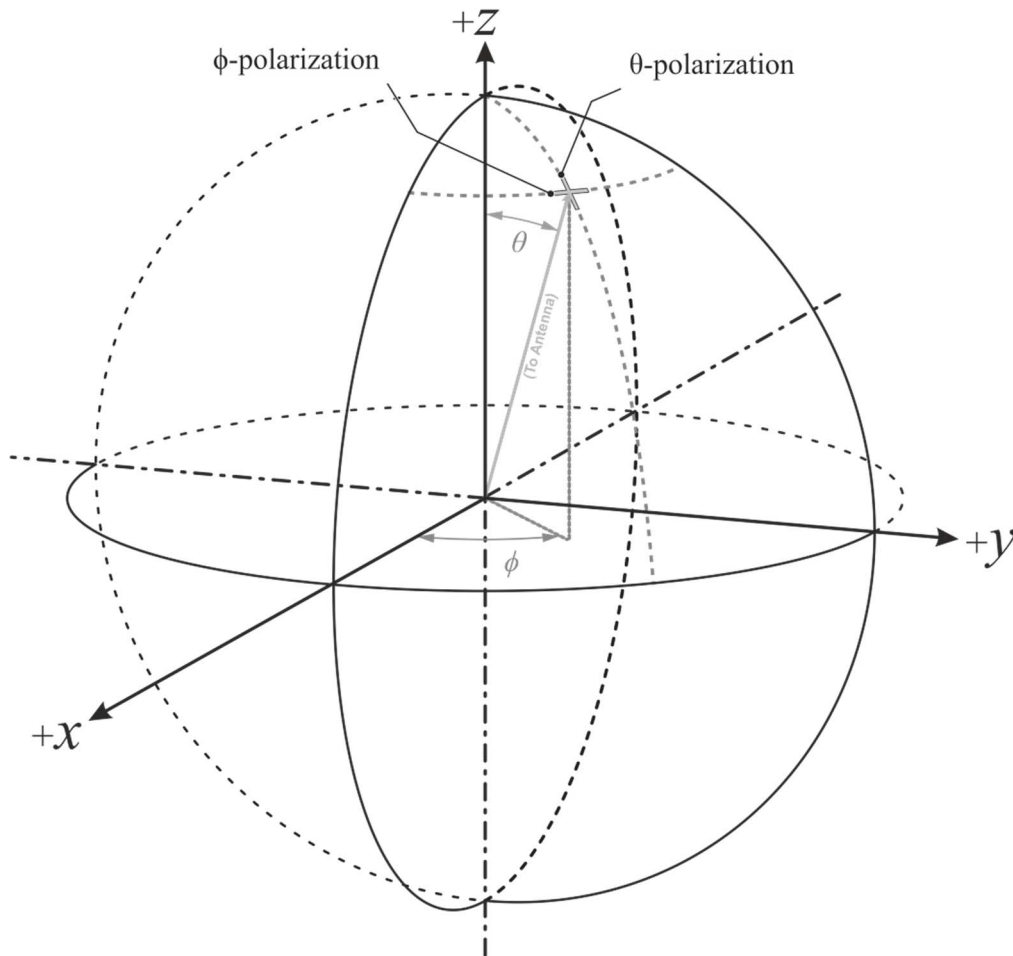
Figure A.4-1: Reference coordinate system
