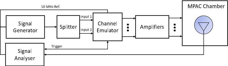
Figure C.3.5-3: Setup for Beam-Specific V/H measurements (Beam 1)
