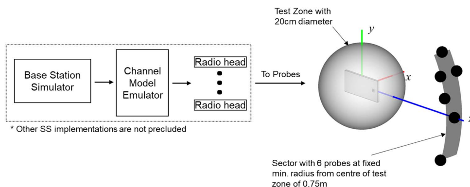
Figure G.2.1-1: 3D MPAC system layout for NR FR2 MIMO OTA testing
