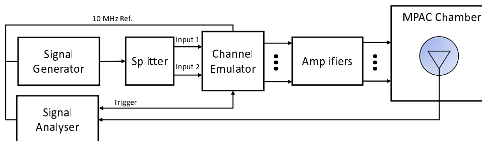
Figure C.3.3-3: Setup for Beam-Specific Doppler measurements (Beam 1)
