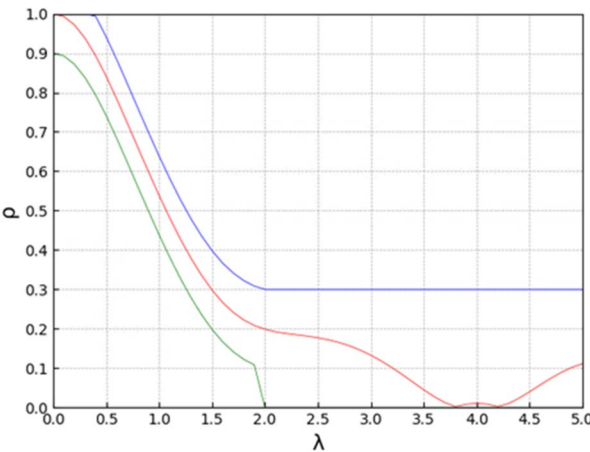
Figure I.4.3-1: Pass/fail limits and targets of Temporal correlation for CDL-C UMi channel model: red curve (reference), blue (upper limit) and green (lower limit)
