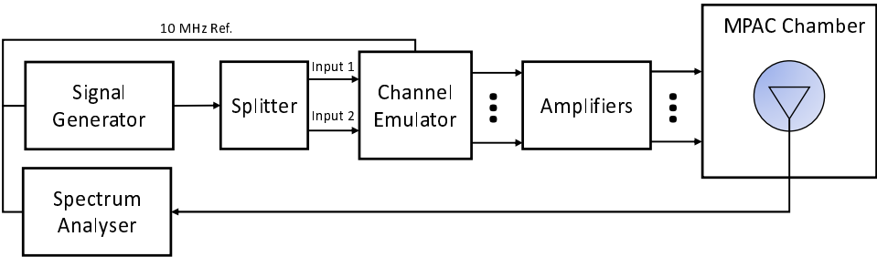
Figure C.3.3-1: Setup for Doppler measurements
