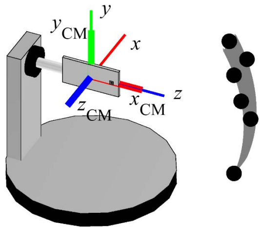
Figure G.2.1-2: Channel Model Coordinate Axes in FR2 3D-MPAC system
