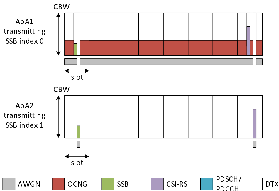
Figure 7.5.1.1.4-2: Time multiplexed downlink transmissions
