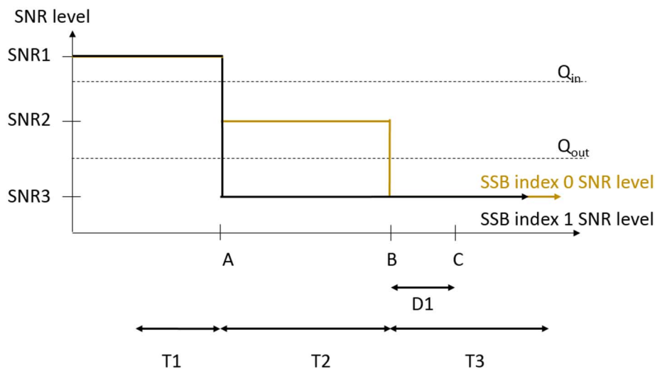
Figure 7.5.1.1.4-1: SNR variation for out-of-sync testing
