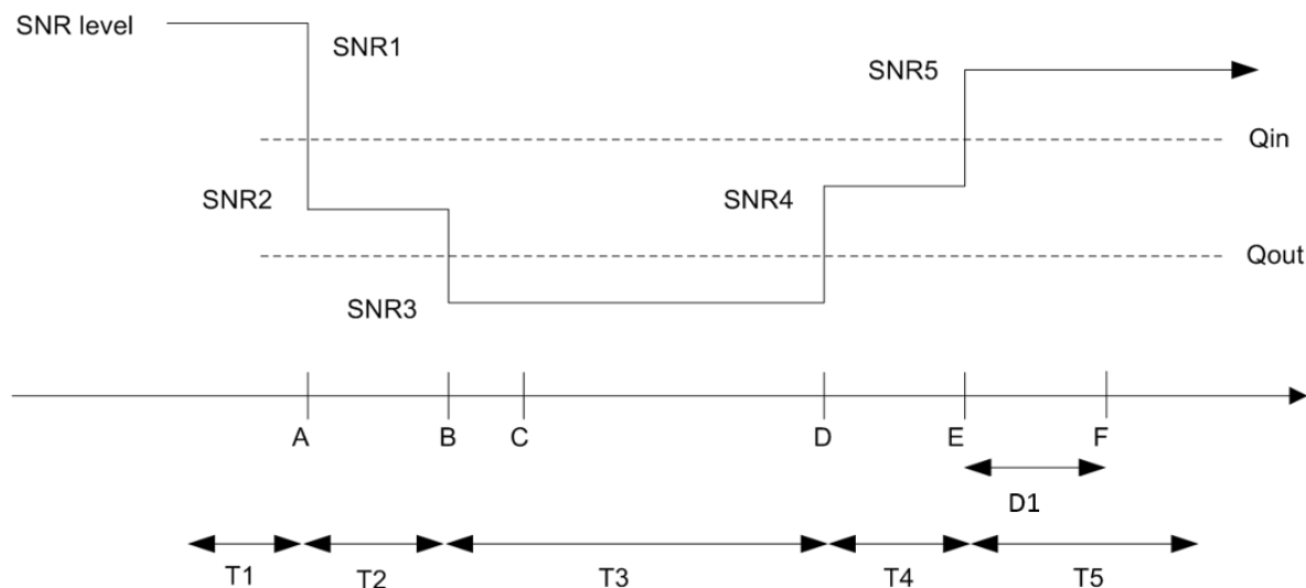
Figure 10.3.1.3.4-1: SNR variation for in-sync testing
