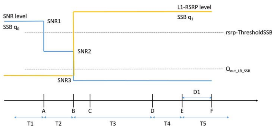
Figure 10.3.4.1.4-1: SNR and L1-RSRP variation for EN-DC FR1 PSCell with CCA Beam Failure Detection and Link Recovery in non-DRX
