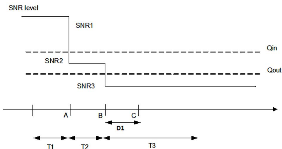
Figure 10.3.1.2.4-1: SNR variation for out-of-sync testing
