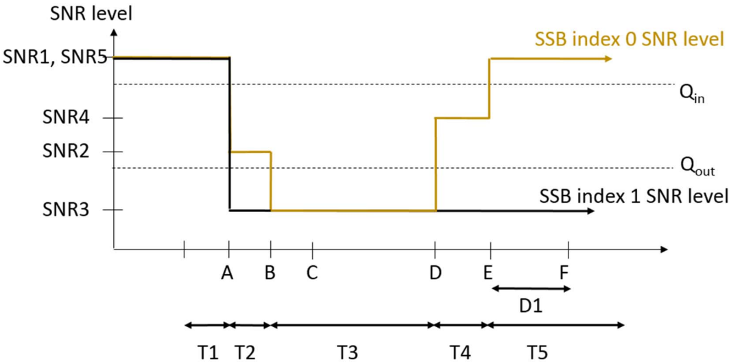
Figure 7.5.1.4.4-1: SNR variation for in-sync testing
