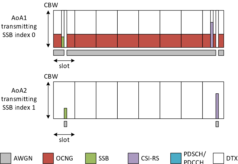
Figure 5.5.1.9.4-1: Time multiplexed downlink transmissions
