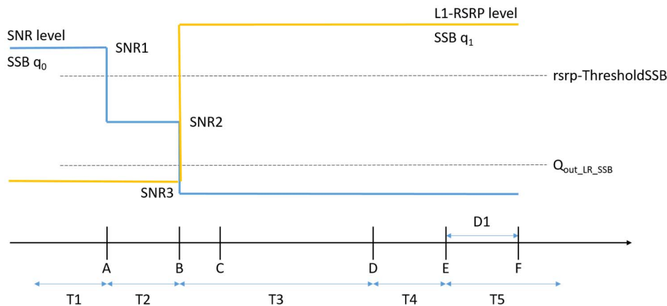
Figure 10.3.4.2.4-1: SNR and L1-RSRP variation for EN-DC FR1 PCell with CCA Beam Failure Detection and Link Recovery in DRX
