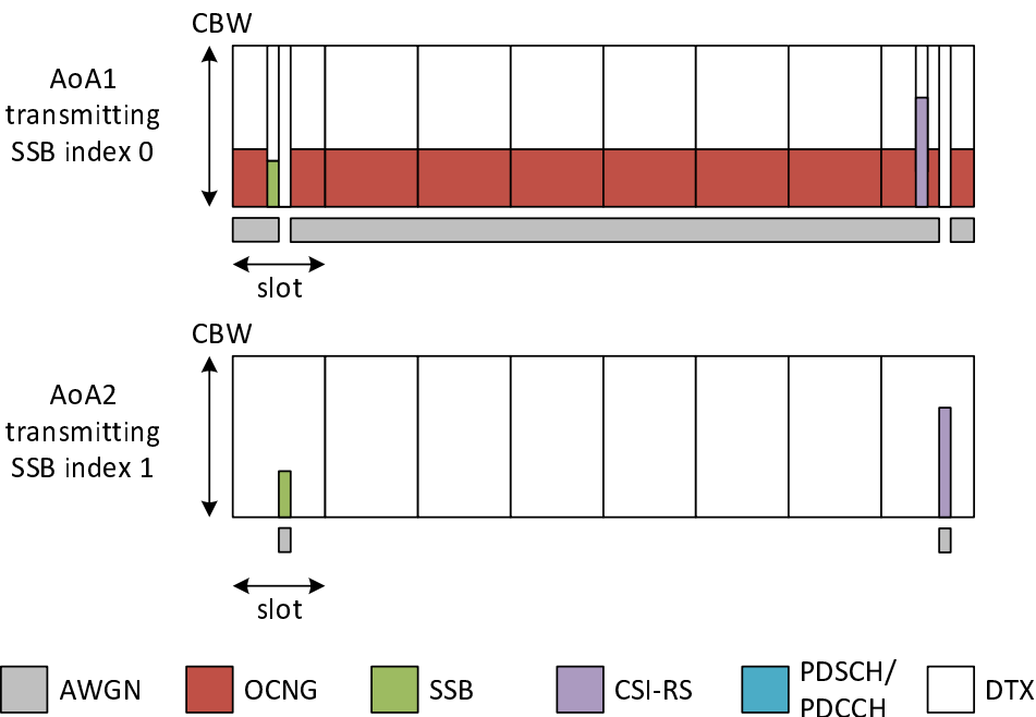
Figure 5.5.1.2.4-2: Time multiplexed downlink transmissions
