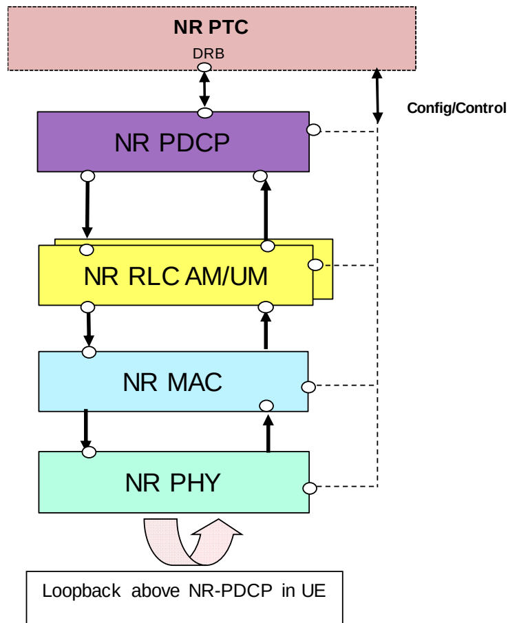
Figure 5.2.2.1-1: Test model for NR/5GC PDCP testing
