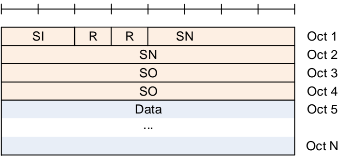
Figure 6.2.2.3-5: UMD PDU with 12 bit SN and with SO
