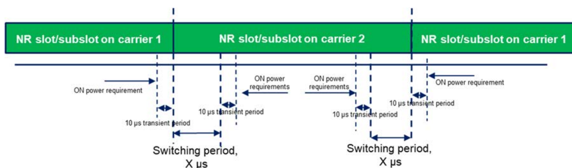
Figure 6.3C.3.0.2-1b: Time mask for switching between SUL carrier 1 and UL Carrier 2, where the switching period is located in carrier 2
