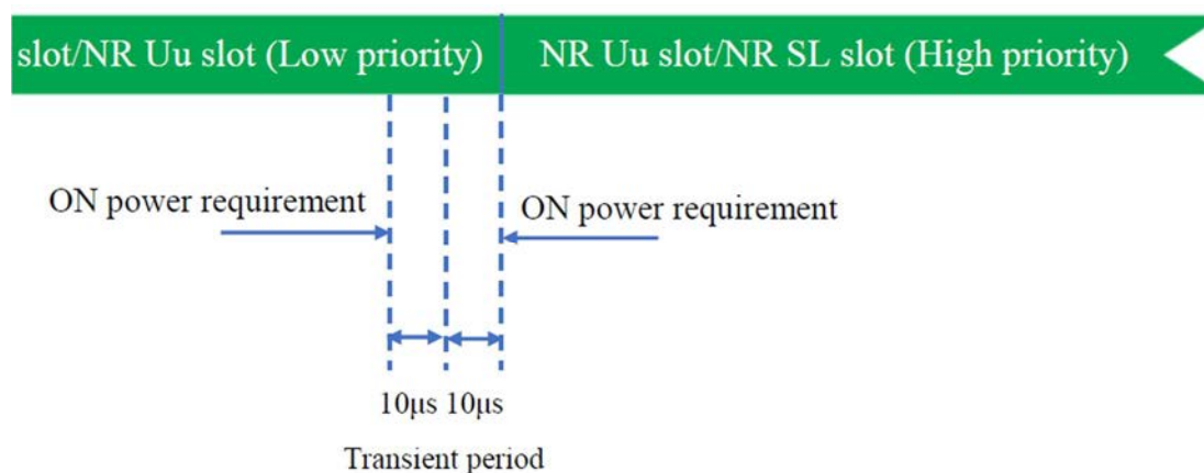
6.3E.3.4-1: Time mask for switching between Uu and SL for same carrier case with same bandwidth
