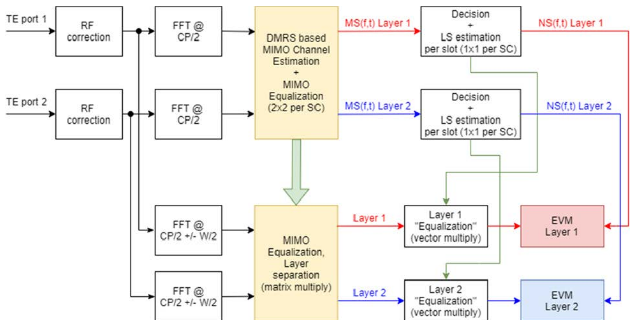
Figure E.8.1-1: EVM calculation block diagram for 2-Layer UL MIMO
