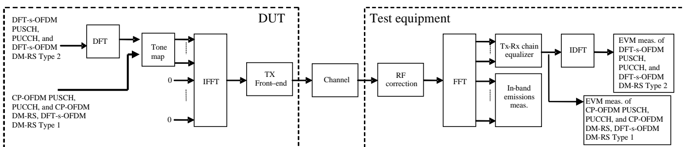
Figure E.2.5-1: EVM measurement points
