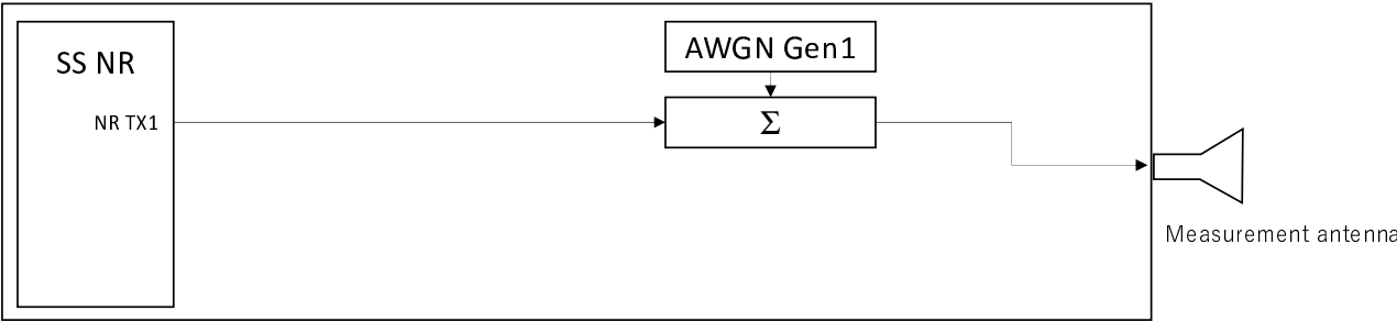
Figure A.3.3.1-1: TE diagram for radiated RRM tests (1x2 without fading)
