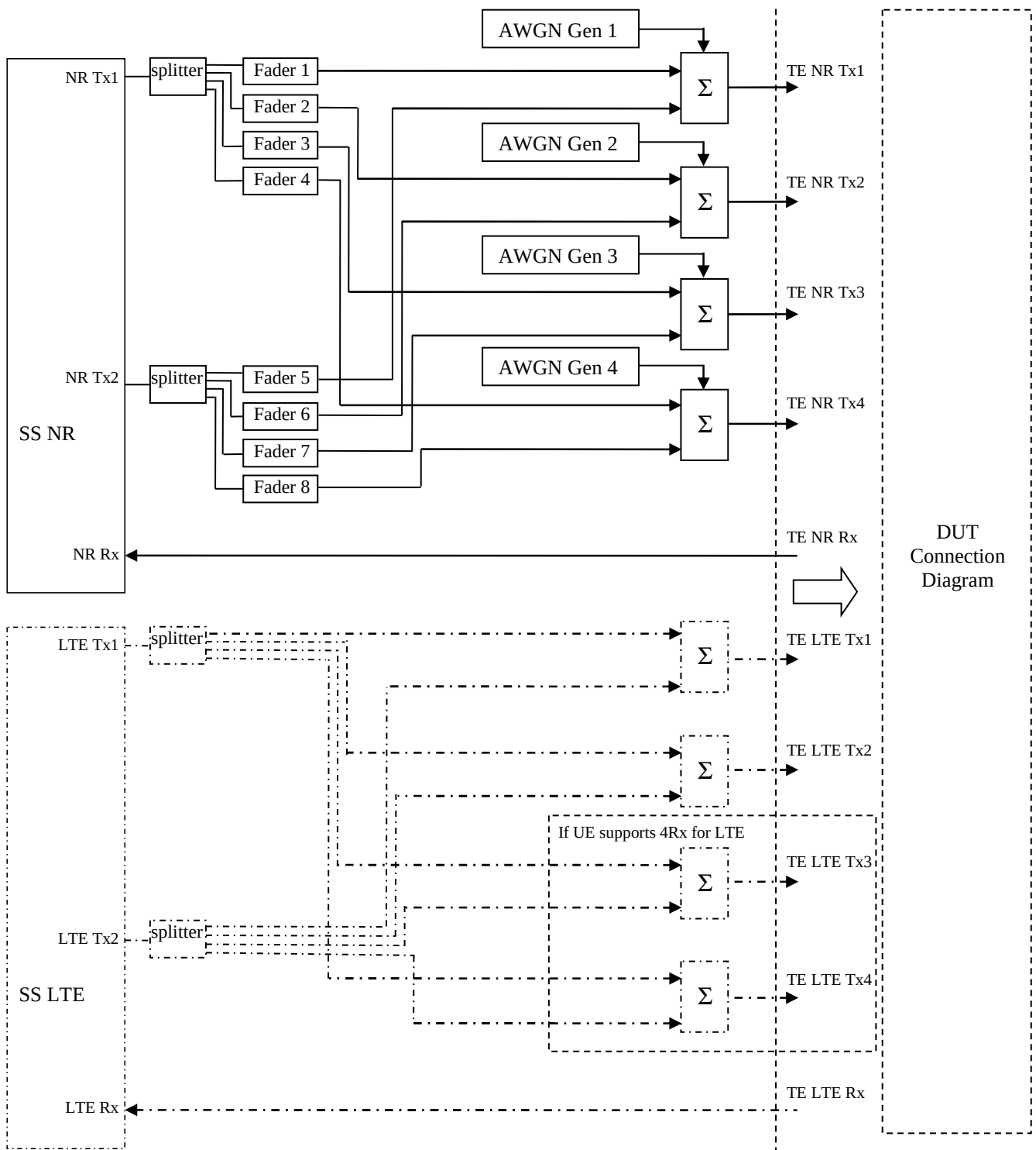
Figure A.3.1.7.4: Test Equipment connection for Demodulation Performance and CSI reporting tests with antenna configuration 2x4
