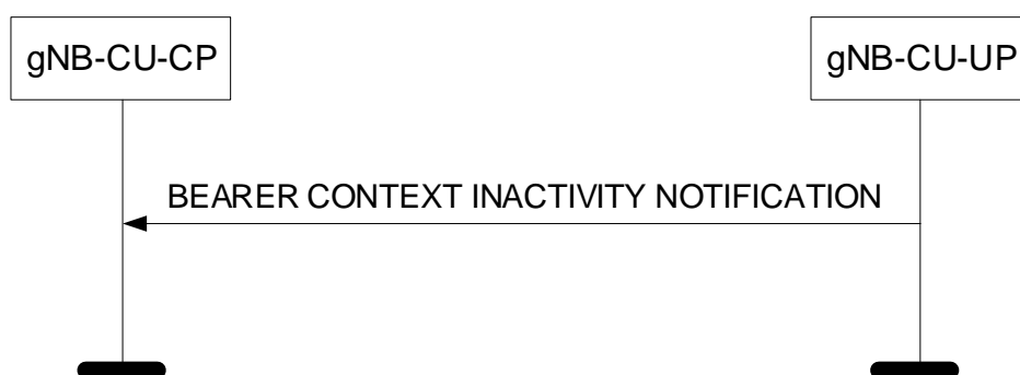
Figure 8.3.6.2-1: Bearer Context Inactivity Notification procedure: Successful Operation.
