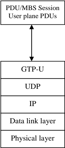
Figure 7.2-1: NG-U protocol structure for PDU/MBS Session
