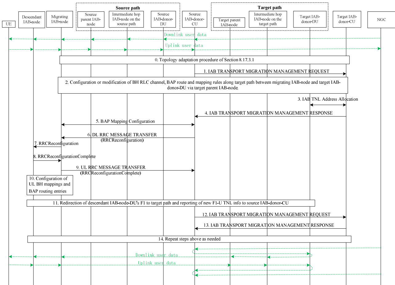
Figure 8.17.3.2-1: IAB inter-CU topology adaptation procedure with descendant IAB-node
