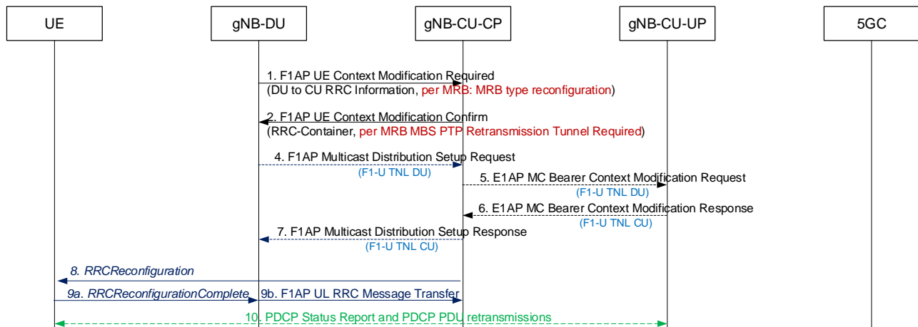
Figure 8.15.1.3-1: Multicast MRB type re-configuration with F1-U ptp retransmission tunnel establishment
