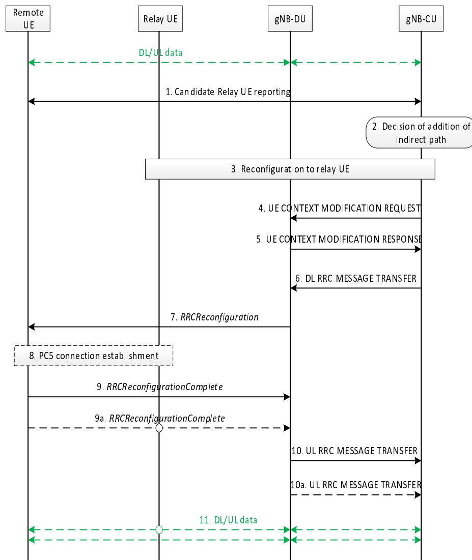
Figure 8.22.4-1: Signalling procedure of intra-DU indirect path addition on top of direct path
