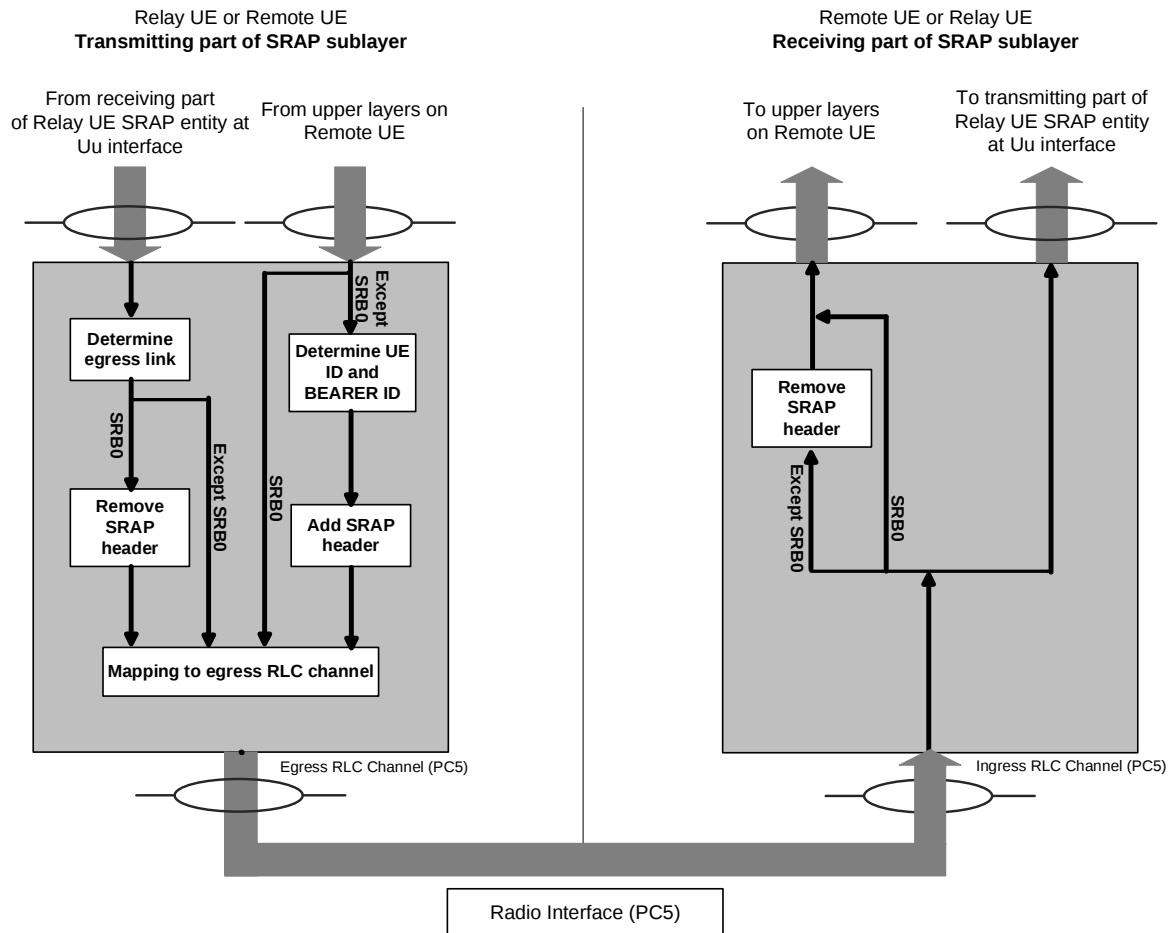
Figure 4.2.2-2: Example of functional view of SRAP sublayer at PC5 interface in U2N Relay case
