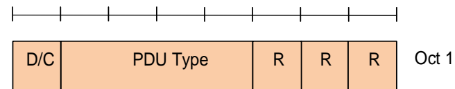
Figure 6.2.3.4-1: BAP Control PDU format for BH RLF detection indication
