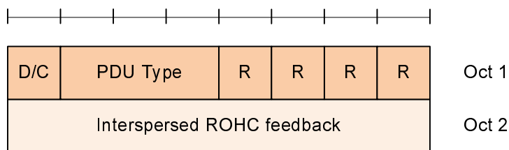
Figure 6.2.3.2-1: PDCP Control PDU format for interspersed ROHC feedback
