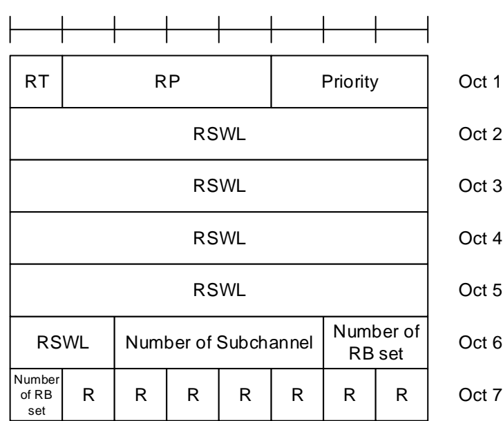
Figure 6.1.3.54-2: Enhanced Inter-UE Coordination Request MAC CE
