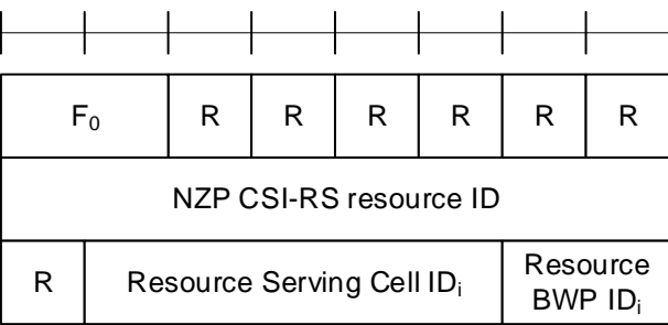
Figure 6.1.3.36-2: Spatial Relation for Resource ID i with NZP CSI-RS
