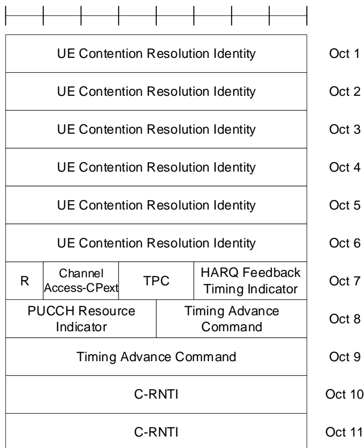
Figure 6.2.3a-2: successRAR
