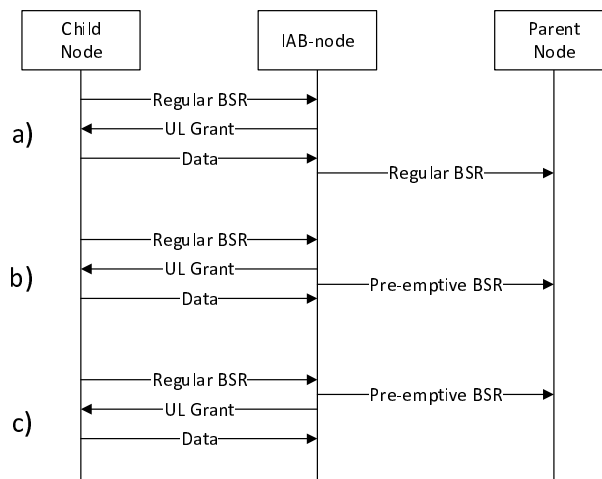
Figure 4.7.3.3-1: Scheduling of BSR in IAB: a) regular BSR based on buffered data, b) Pre-emptive BSR based on UL grant, c) Pre-emptive BSR based on reception of regular BSR
