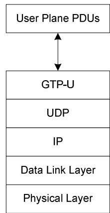
Figure 4.3.1.1-1: NG-U Protocol Stack
