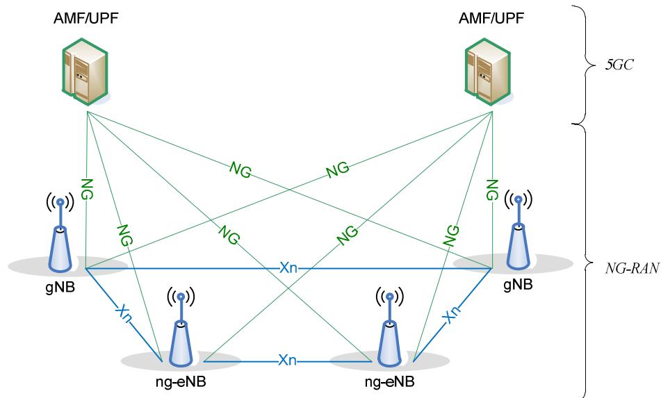
Figure 4.1-1: Overall Architecture
