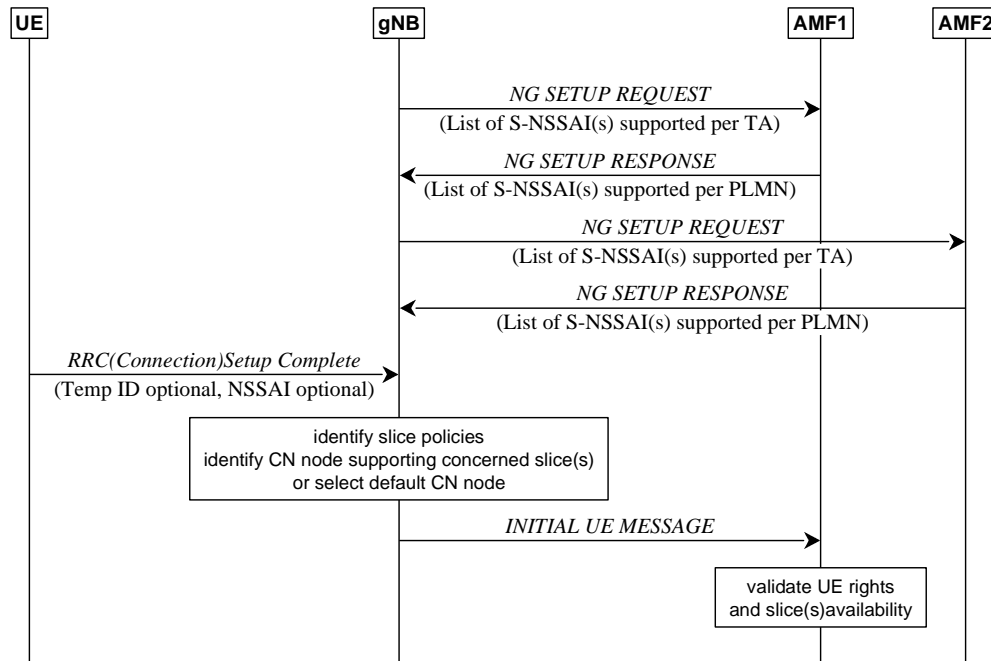
Figure 16.3.4.2-1: AMF selection
