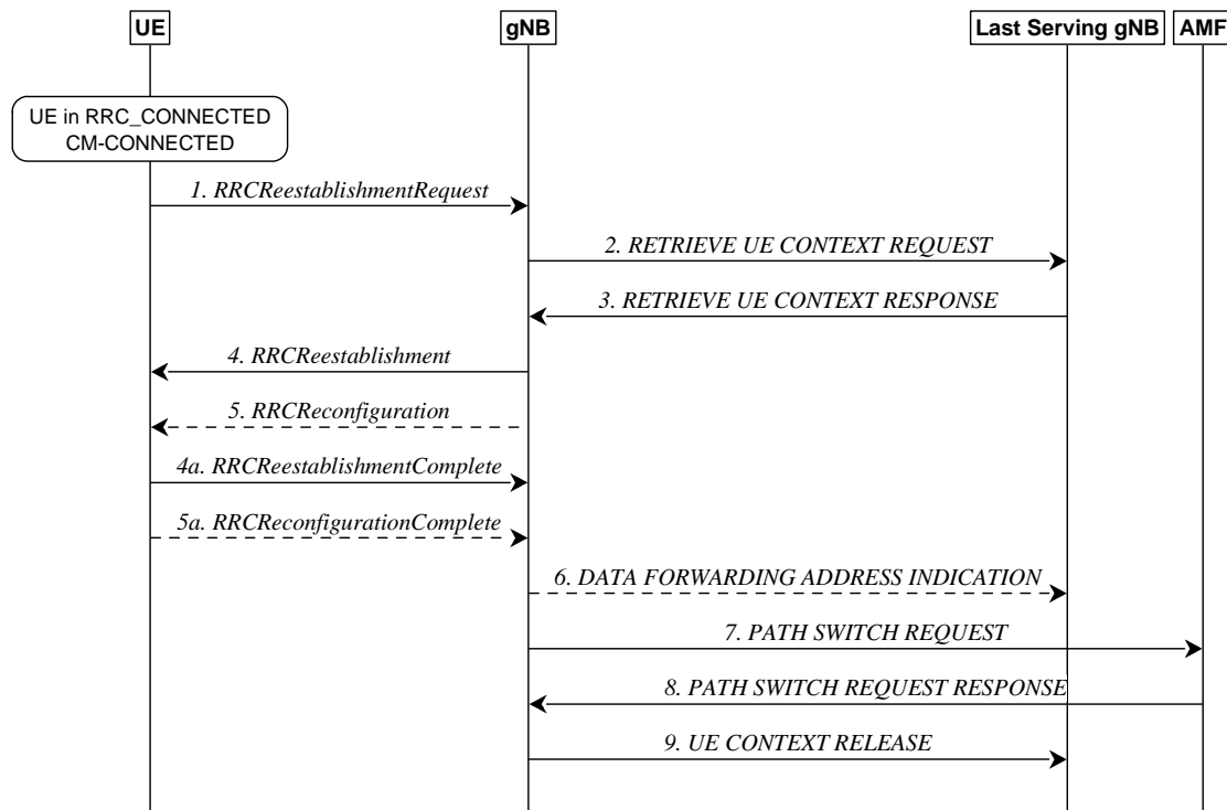
Figure 9.2.3.3-1: Re-establishment procedure
