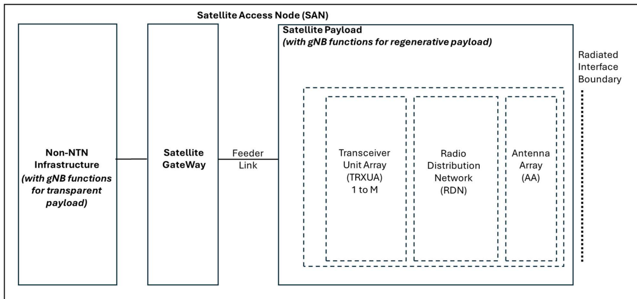
Figure 4.2.2-1: Radiated reference points for SAN type 1-O and SAN type 2-O
