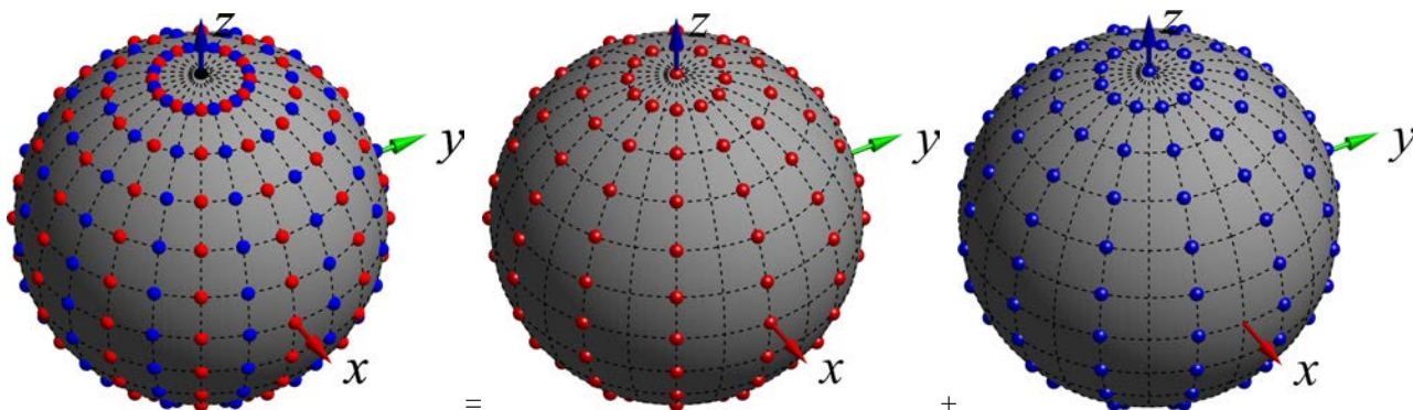
Figure A.3.3.4-3: Split 3x89 measurement grids,
