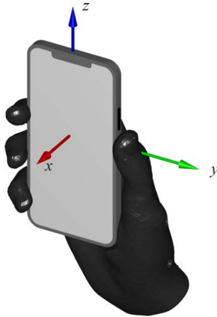
Figure B.3.5-1: Hand phantom only for NTN scenario 2 (default, i.e., elevation tilt 0°)
