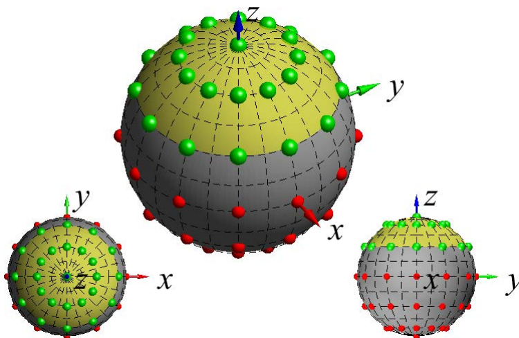
Figure D.2.5.1-1: Visualization of partial surface with ±60° angular width for classical TRS grid.
