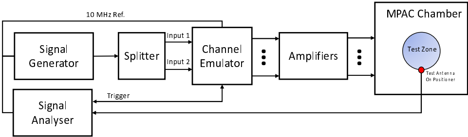
Figure C.3.4-6: Configuration for spatial correlation validation based on time domain techniques
