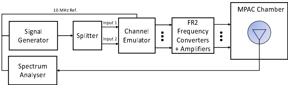
Figure D.3.3-1: Setup for FR2 Doppler measurements
