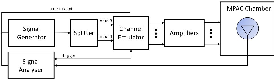
Figure C.3.5-4: Setup for Beam-Specific V/H measurements (Beam 2 CDL-C UMa only)
