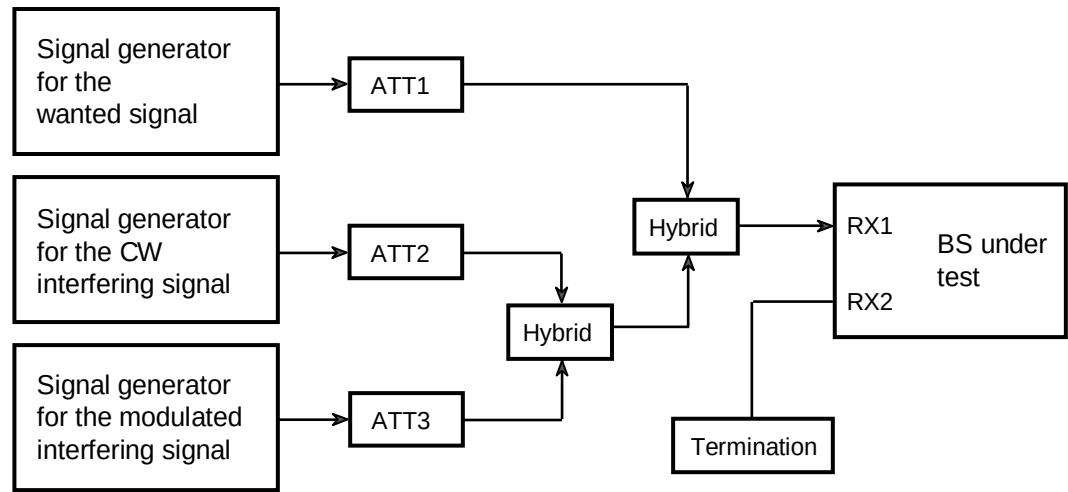
Figure D.2.7-1: Measuring system set-up for BS type 1-C intermodulation characteristics
