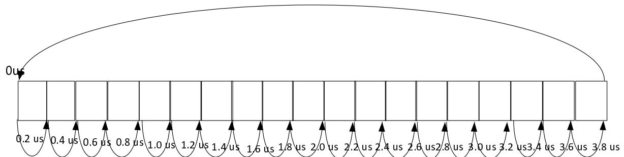
Figure 8.2.9.4.2-2: Timing offset scheme for MsgA transmission for BS type 1-C and type 1-H with 15 kHz SCS
