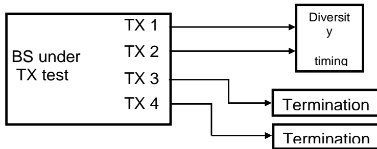
Figure D.1.3-1: Measuring system set-up for BS type 1-C test of time alignment error
