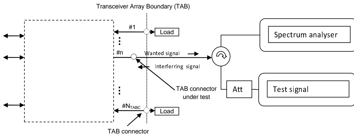
Figure D.3.2-1: Measuring system set-up for BS type 1-H transmitter intermodulation
