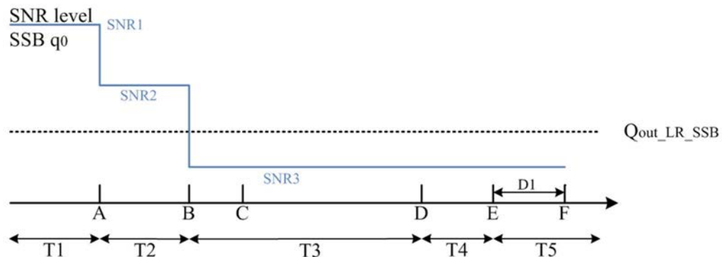
Figure A.17.5.2.2.1-1: SNR variation for SSB-based beam failure detection and link recovery testing in DRX mode
