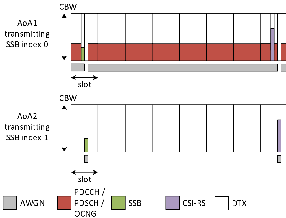
Figure A.5.11.3.1.1-1: Time multiplexed downlink transmissions during T1
