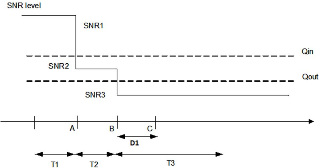
Figure A.14.4.1.3.1-1: SNR variation for out-of-sync testing
