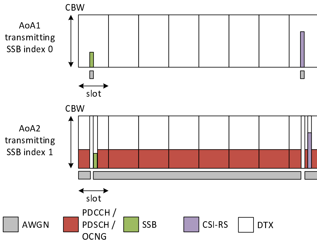
Figure A.17.5.4.2.1.1-2: Time multiplexed downlink transmissions during T2
