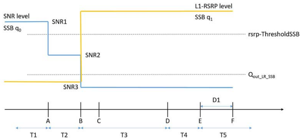
Figure A.16.5.2.4.1-1: SNR and L1-RSRP variation for SSB-based beam failure detection and link recovery testing in non-DRX mode
