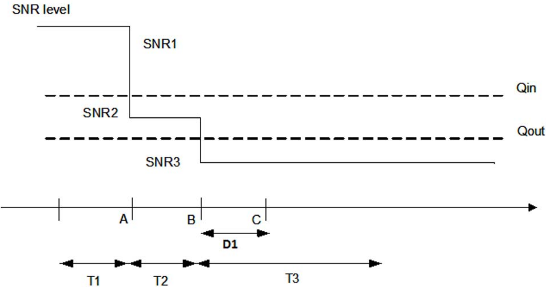
Figure A.16.5.1.5.1-1: SNR variation for out-of-sync testing
