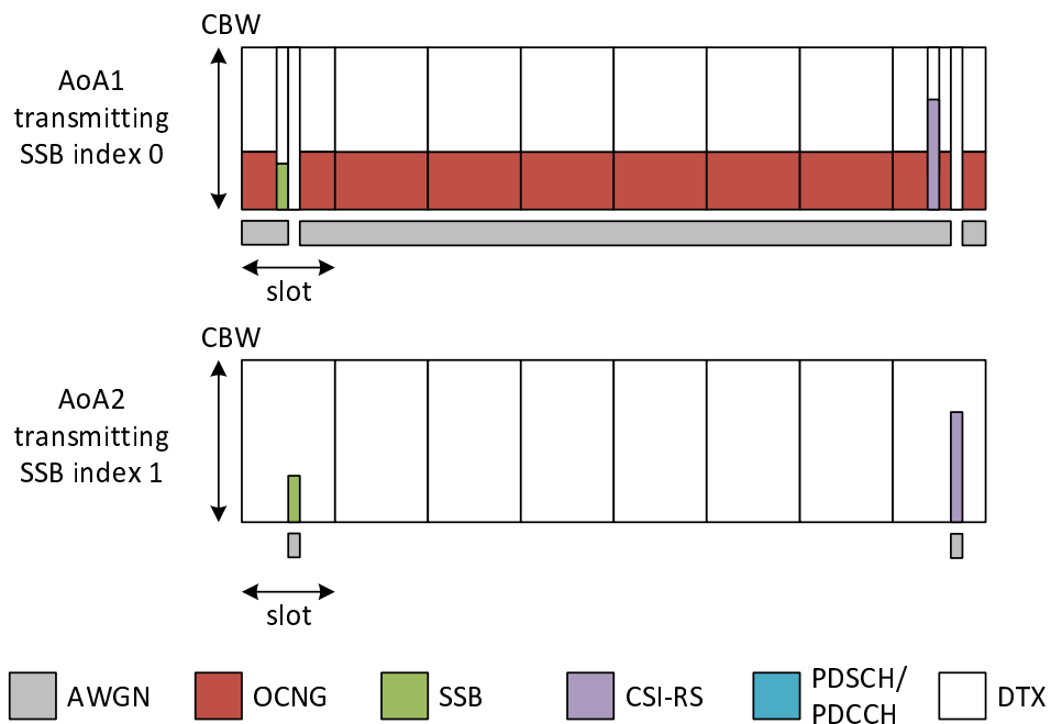
Figure A.17.5.1.1 .1-2: Time multiplexed downlink transmissions
