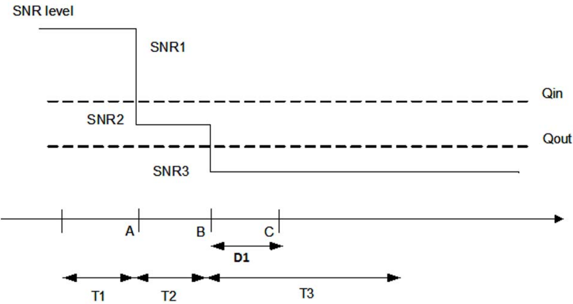
Figure A.16.5.1.1.1-1: SNR variation for out-of-sync testing
