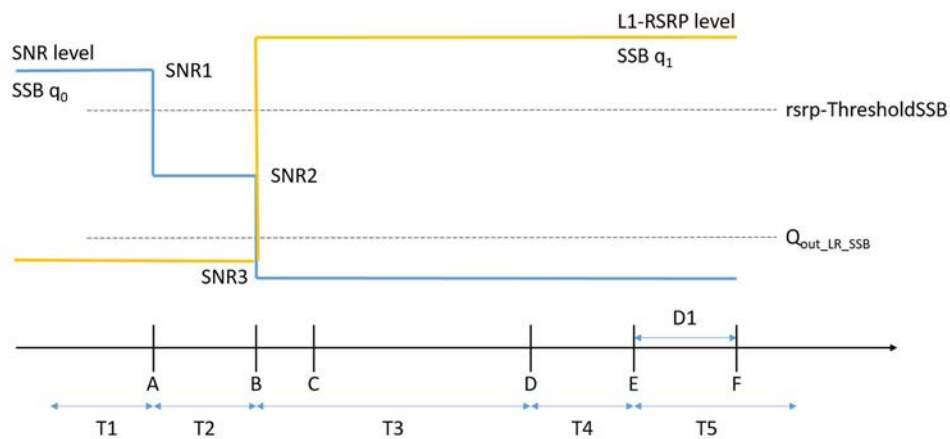
Figure A.16.5.2.2.1-1: SNR and L1-RSRP variation SSB for SSB-based beam failure detection and link recovery testing in non-DRX mode
