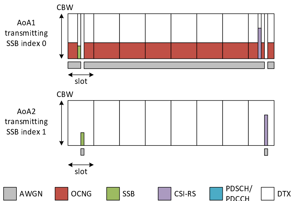
Figure A.17.5.1.2.1-2: Time multiplexed downlink transmissions
