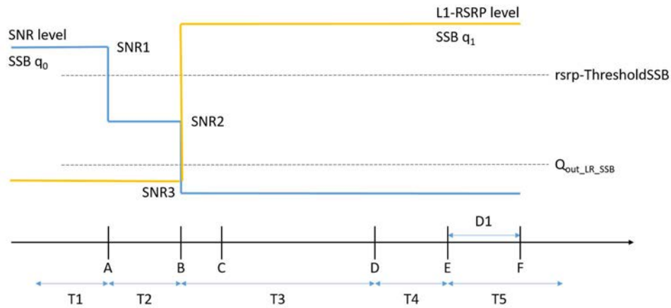
Figure A.14.4.2.1.1-1: SNR and L1-RSRP variation SSB for SSB-based beam failure detection and link recovery testing in non-DRX mode
