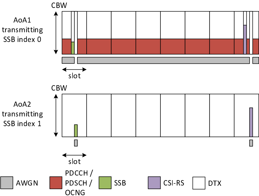
Figure A.17.5.4.1.1-1: Time multiplexed downlink transmissions during T1
