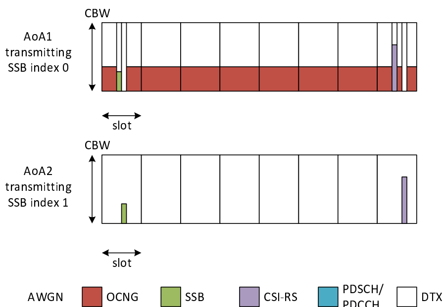
Figure A.7.6.1.6.1-1: Time multiplexed downlink transmissions (Config 1 example)
