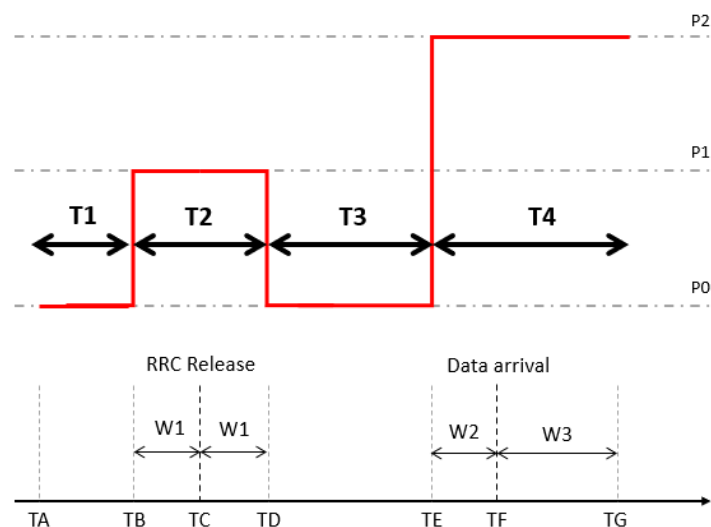
Figure A.7.2.1.1-1: RSRP variation for TA validation for CG-SDT Sub-test#1
