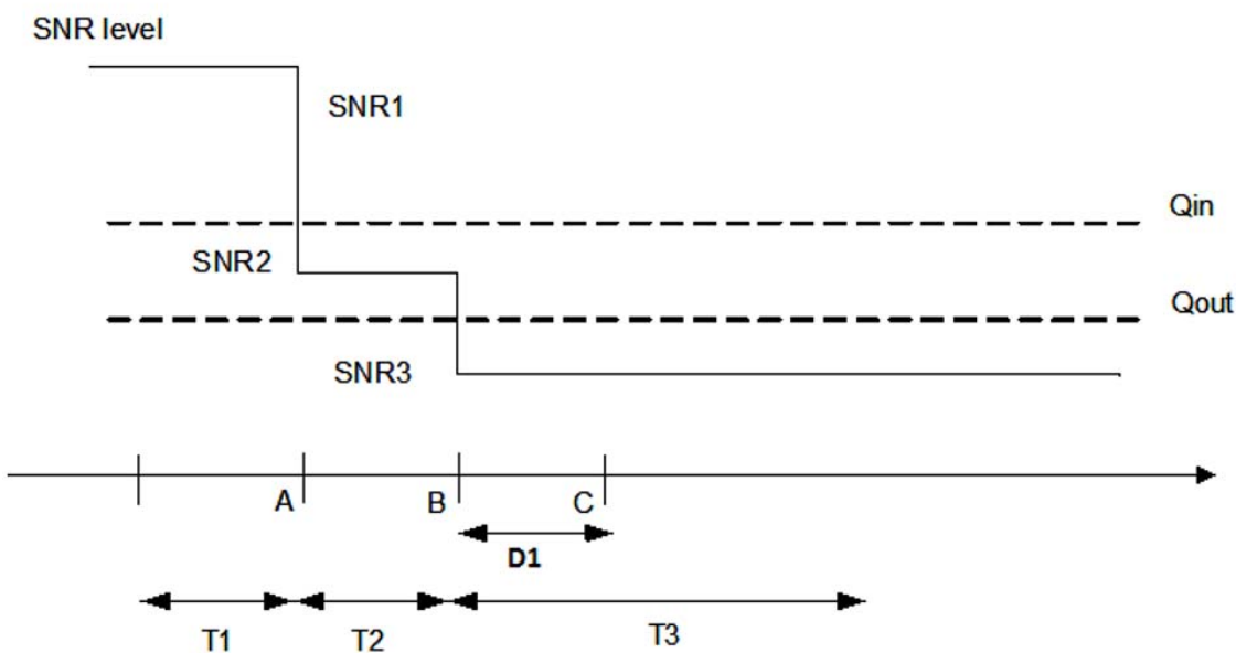
Figure A.16.5.1.6.1-1: SNR variation for out-of-sync testing
