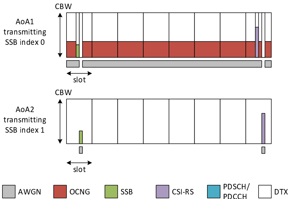
Figure A.17.5.1.9.1-1: Time multiplexed downlink transmissions
