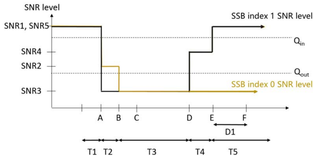
Figure A.17.5.1.2.1-1: SNR variation for in-sync testing
