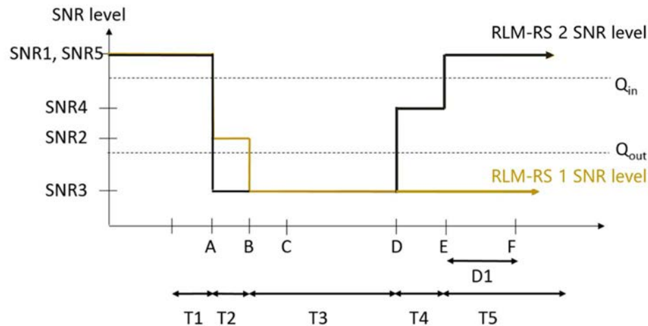
Figure A.17.5.1.6.1-1: SNR variation for CSI-RS in-sync testing
