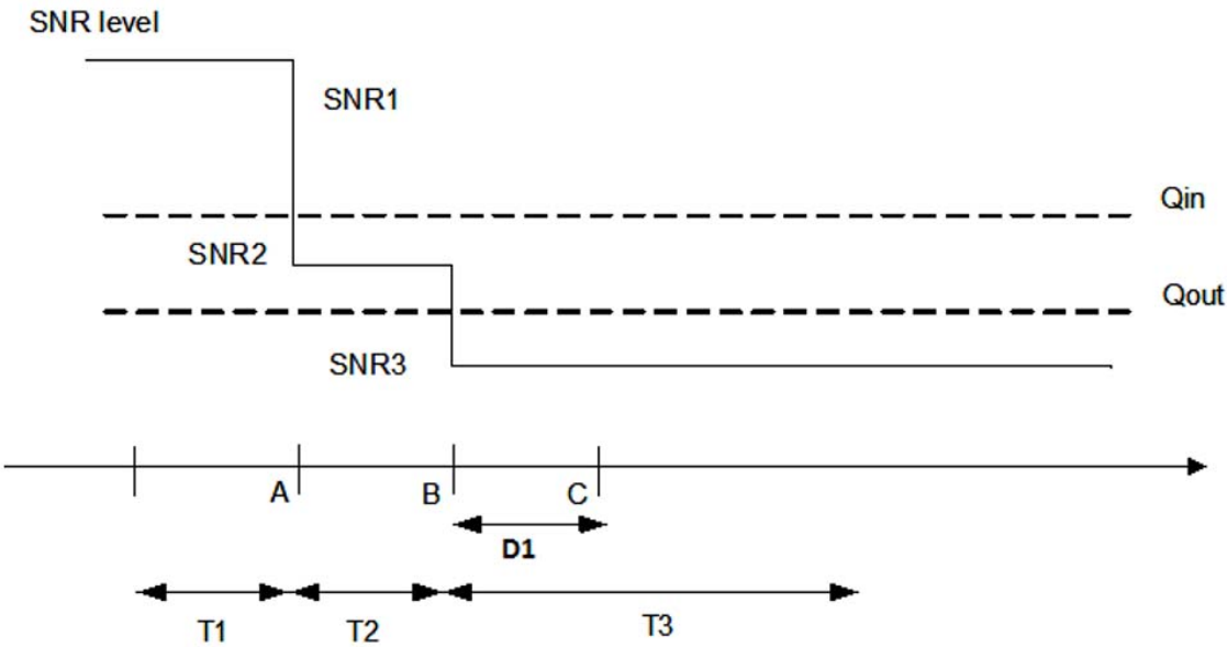
Figure A.16.5.1.2.1-1: SNR variation for out-of-sync testing
