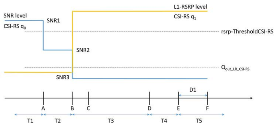
Figure A.14.4.2.3.1-1: SNR and L1-RSRP variation for CSI-RS-based beam failure detection and link recovery testing in non-DRX mode
