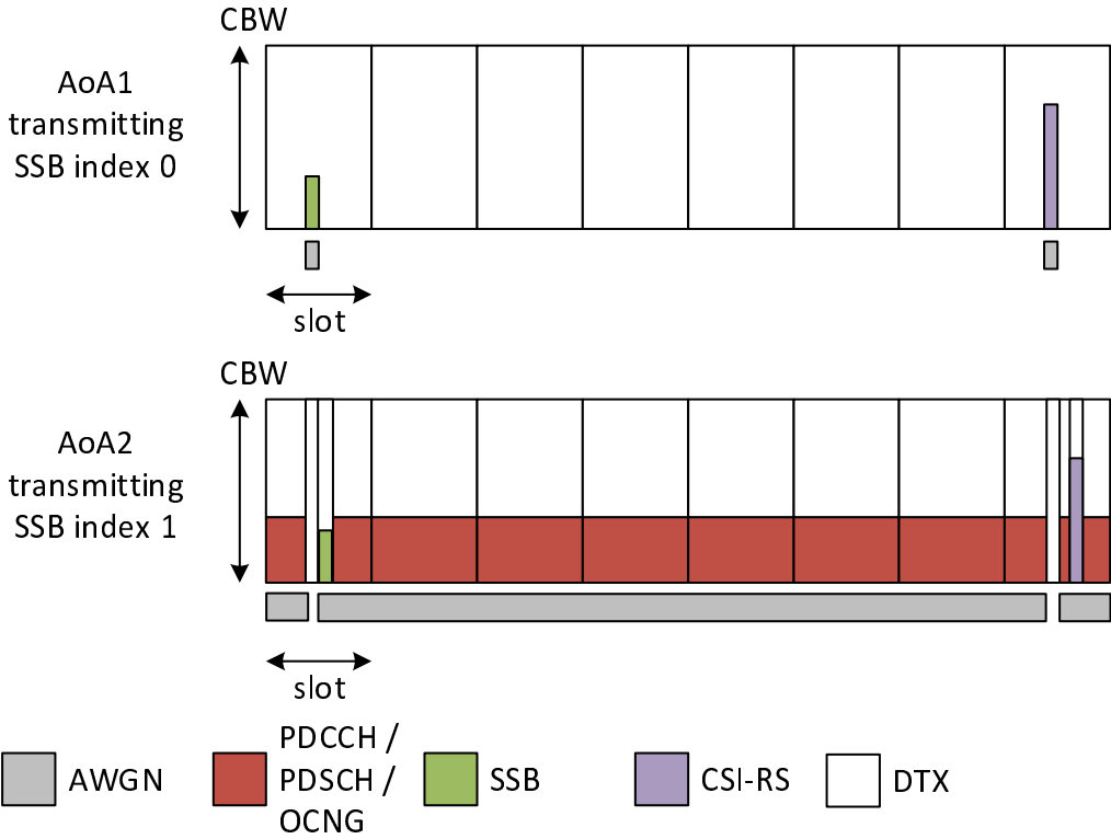
Figure A.17.5.4.1.1-2: Time multiplexed downlink transmissions during T2
