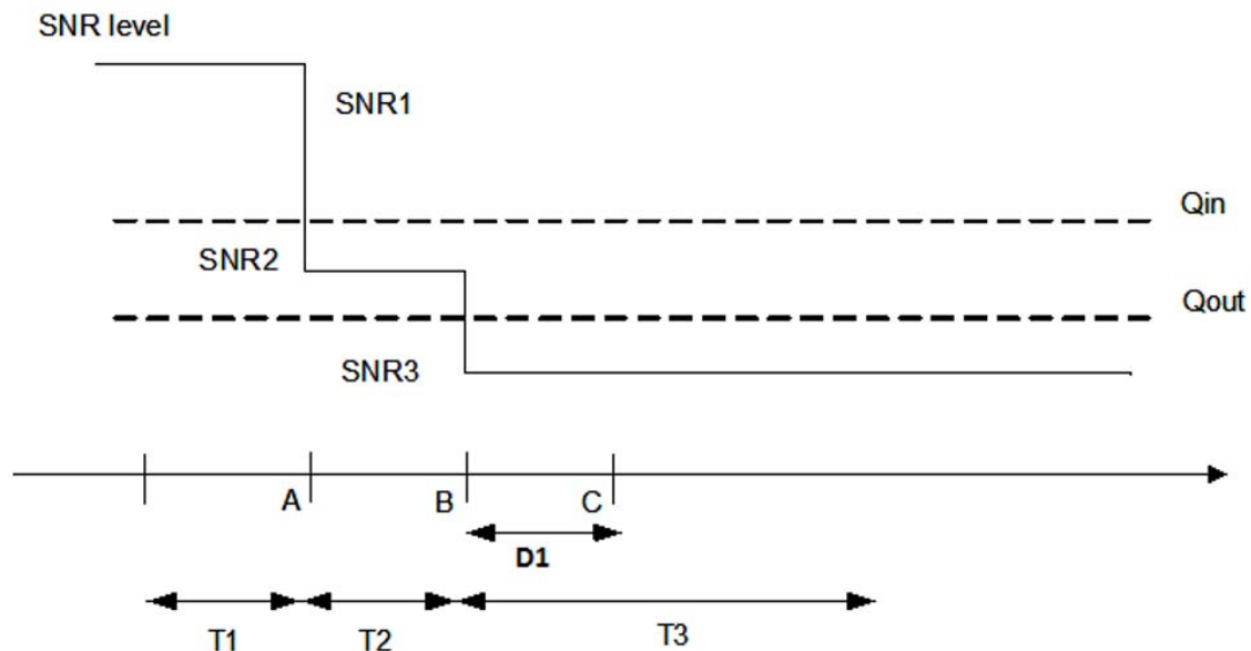
Figure A.14.4.1.1.1-1: SNR variation for out-of-sync testing
