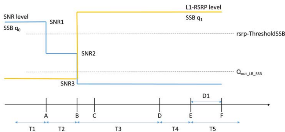
Figure A.16.5.2.1.1-1: SNR and L1-RSRP variation SSB for SSB-based beam failure detection and link recovery testing in non-DRX mode
