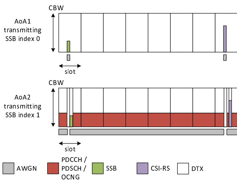
Figure A.7.5.8.3.1.1-2: Time multiplexed downlink transmissions during T2
