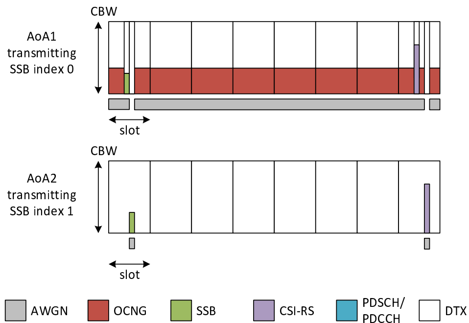
Figure A.17.5.1.3.1-2: Time multiplexed downlink transmissions
