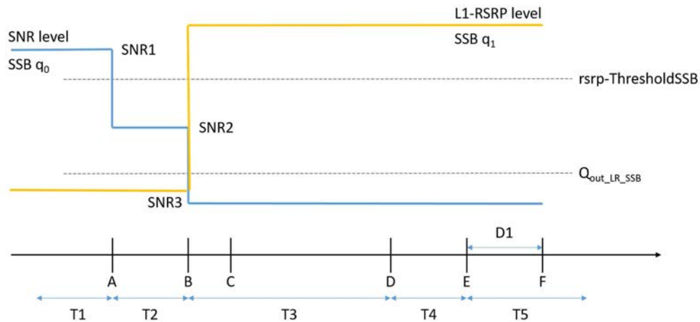
Figure A.11.4.4.2.1-1: SNR and L1-RSRP variation for SSB-based beam failure detection and link recovery testing in non-DRX mode
