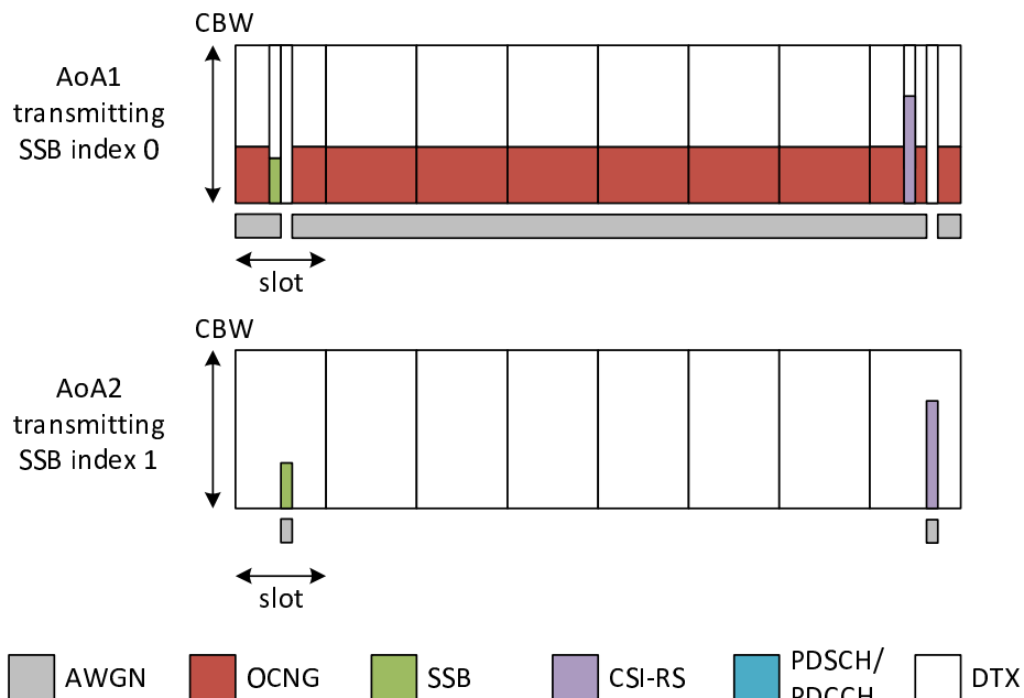
Figure A.7.5.1.2.1-1: SNR variation for in-sync testing
