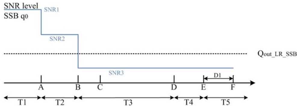
Figure A.5.5.5.1.1-1: SNR variation for SSB-based beam failure detection and link recovery testing in non-DRX mode
