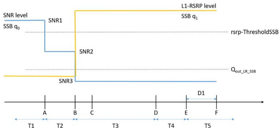
Figure A.11.4.2.1-1: SNR and L1-RSRP variation for SSB-based beam failure detection and link recovery testing in non-DRX mode
